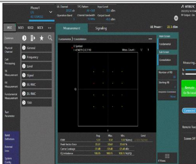
Band5-10MHz-16QAM-20525-50RB#0
