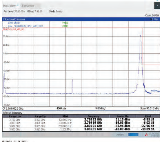
1-N78-3700-3800--30-80-H-2-DFT-PI2BPSK-Edge_1R_B_Right-1@216-Ant1-PASS-see graph
