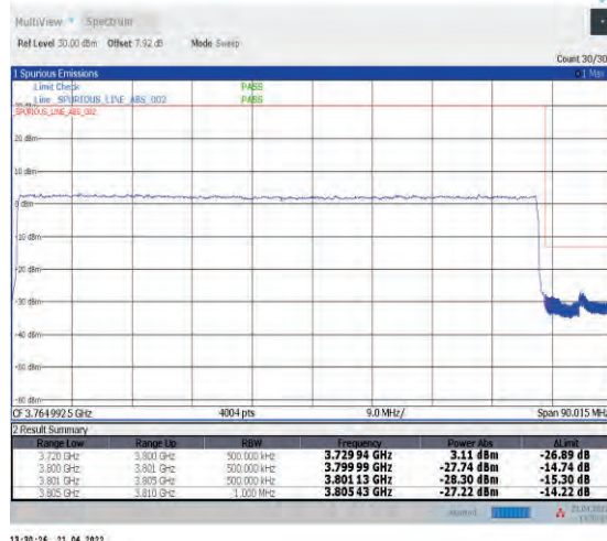
1-N78-3700-3800--30-80-H-3-DFT-PI2BPSK-Outer_Full-216@0-Ant1-PASS-see graph
