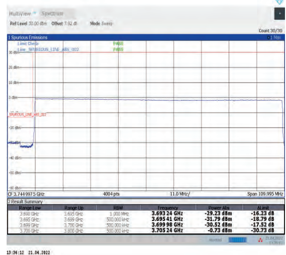
1-N78-3700-3800--30-100-L-6-CP-QPSK-Outer_F ull-273@0-Ant1-PASS-see graph
