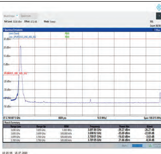
1-N78-3700-3800-PC1-30-90-L-1-DFT-PI2BPSK-Edg_e_1RB_Left-1@0-Ant1-1--PASS-see graph
