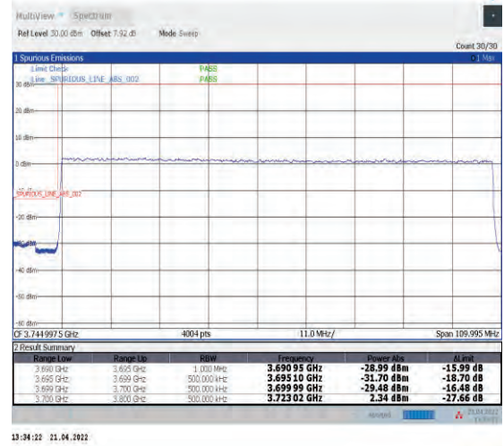
1-N78-3700-3800--30-100-L-3-DFT-PI2BPSK-Out er_Full-270@0-Ant1-PASS-see graph
