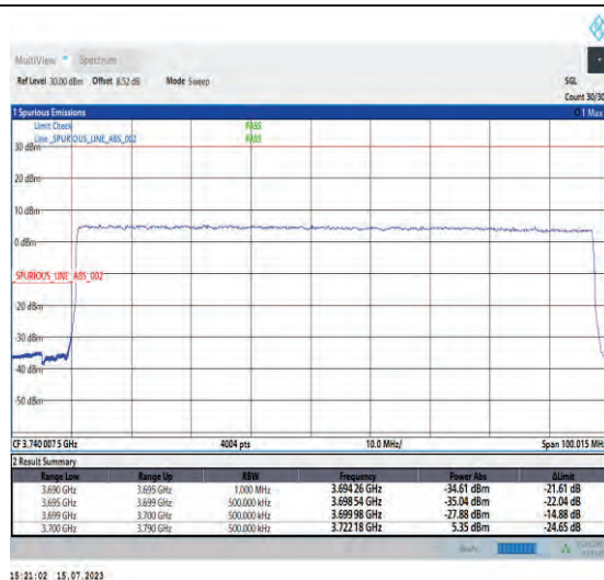
1-N78-3700-3800-PC1-30-90-L-3-DFT-PI2BPSK-Outer_Full-240@0-Ant1-1--PASS-see graph
