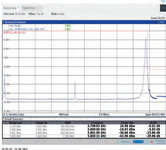
1-N78-3700-3800--30-80-H-5-CP-QPSK-Edge_1RB_Right-1@216-Ant1-PASS-see graph
