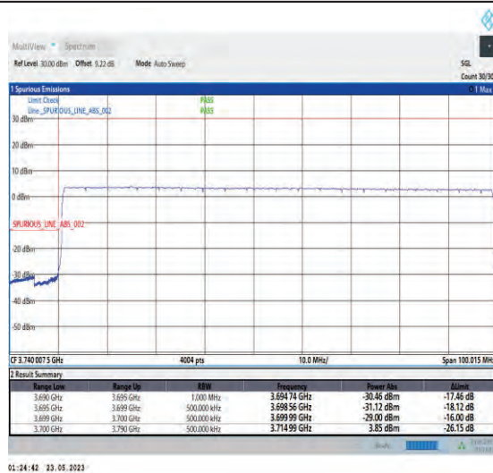
1-N78-3700-3800-PC1-30-90-L-6-CP-QPSK-Outer_Full-245@0-Ant1-1--PASS-see graph
