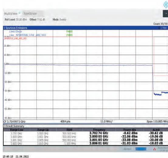
1-N78-3700-3800--30-100-H-6-CP-QPSK-Outer_Full-273@0-Ant1-PASS-see graph
