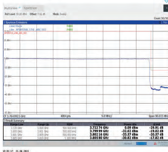
1-N78-3700-3800--30-80-H-6-CP-QPSK-Outer_Full-217@0-Ant1-PASS-see graph
