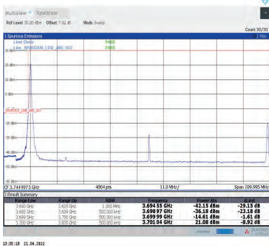
1-N78-3700-3800--30-100-L-4-CP-QPSK-Edge_1RB_ Left-1@0-Ant1-PASS-see graph
