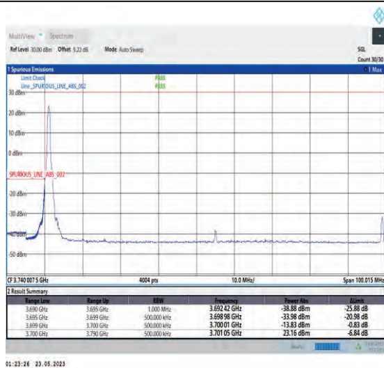
1-N78-3700-3800-PC1-30-90-L-4-CP-QPSK-Edge_1RB_Left-1@0-Ant1-1--PASS-see graph
