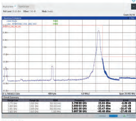
1-N78-3700-3800--30-30-H-5-CP-QPSK-Edge_1RB_R ight-1@77-Ant1-PASS-see graph
