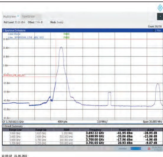
1-N78-3700-3800--30-20-L-1-DFT-PI2BPSK-Edge_1R_B_Left-1@0-Ant1-PASS-see graph
