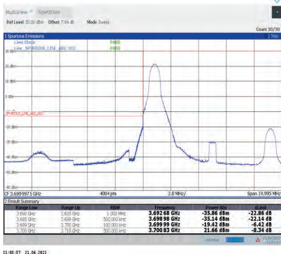
1-N78-3700-3800--30-10-L-4-CP-QPSK-Edge_1RB_L eft-1@0-Ant1-PASS-see graph
