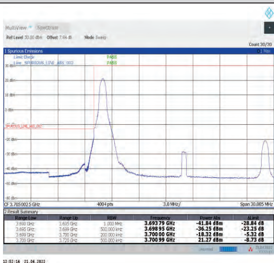
1-N78-3700-3800--30-20-L-4-CP-QPSK-Edge_1RB_L eft-1@0-Ant1-PASS-see graph
