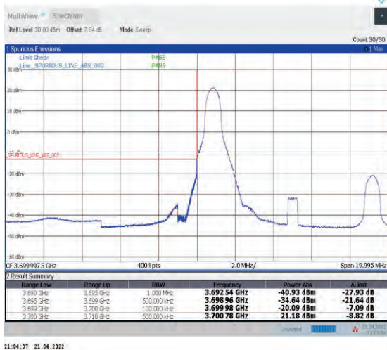
1-N78-3700-3800--30-10-L-1-DFT-PI2BPSK-Edge_1R B_Left-1@0-Ant1-PASS-see graph
