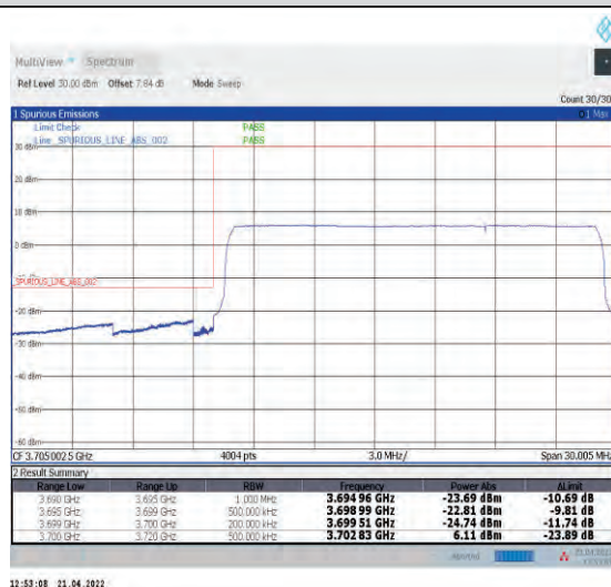
1-N78-3700-3800--30-20-L-6-CP-QPSK-Outer_Ful l-51@0-Ant1-PASS-see graph
