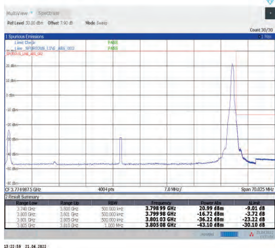
1-N78-3700-3800--30-60-H-5-CP-QPSK-Edge_1RB_Right-1@161-Ant1-PASS-see graph
