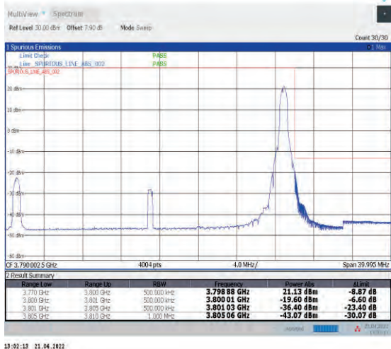
1-N78-3700-3800--30-30-H-2-DFT-PI2BPSK-Edge_1R B_Right-1@77-Ant1-PASS-see graph
