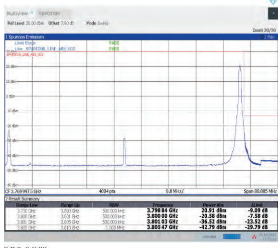
1-N78-3700-3800--30-70-H-5-CP-QPSK-Edge_1RB_Right-1@188-Ant1-PASS-see graph
