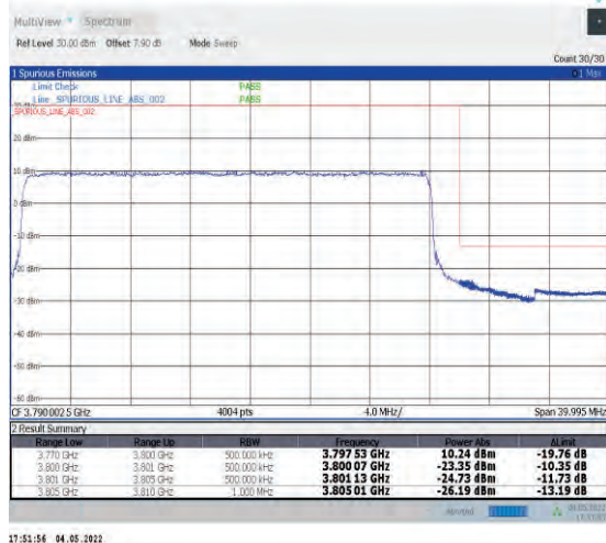
1-N78-3700-3800--30-30-H-3-DFT-PI2BPSK-Outer _Full-75@0-Ant1-PASS-see graph
