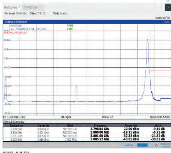
1-N78-3700-3800--30-70-H-2-DFT-PI2BPSK-Edge_1R_B_Right-1@188-Ant1-PASS-see graph
