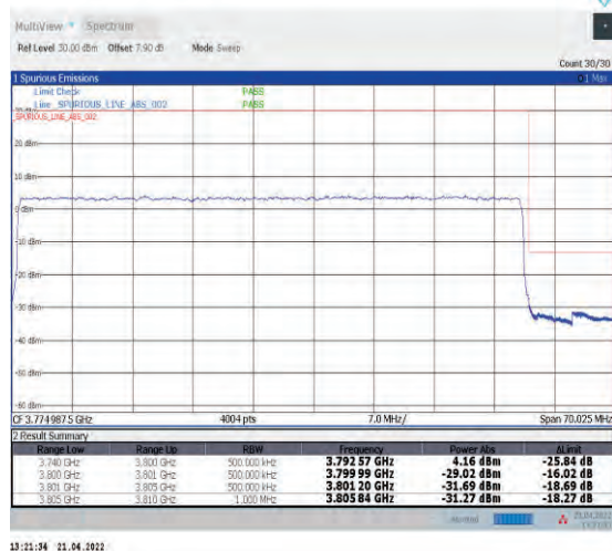
1-N78-3700-3800--30-60-H-3-DFT-PI2BPSK-Outer_Full-162@0-Ant1-PASS-see graph
