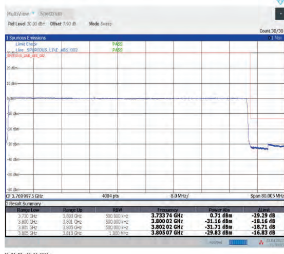
1-N78-3700-3800--30-70-H-6-CP-QPSK-Outer_Full-189@0-Ant1-PASS-see graph
