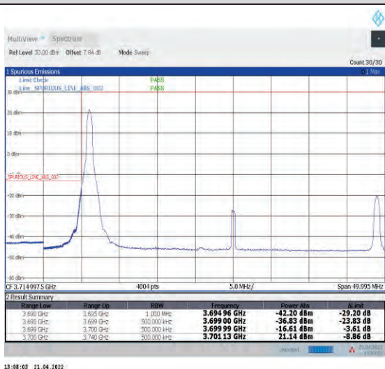
1-N78-3700-3800--30-40-L-4-CP-QPSK-Edge_1RB_L_eff-1@0-Ant1-PASS-see graph
