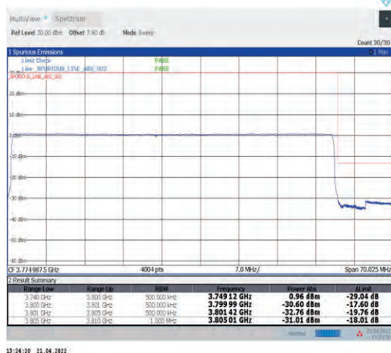
1-N78-3700-3800--30-60-H-6-CP-QPSK-Outer_Full-162@0-Ant1-PASS-see graph
