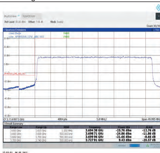
1-N78-3700-3800--30-40-L-3-DFT-PI2BPSK-Outer_Full-100@0-Ant1-PASS-see graph
