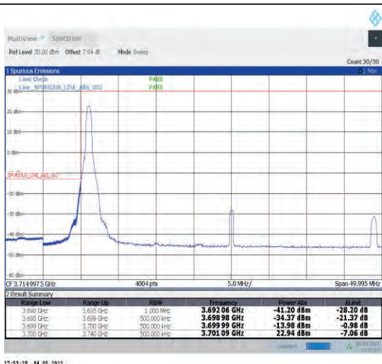
1-N78-3700-3800--30-40-L-1-DFT-PI2BPSK-Edge_1R_B_Left-1@0-Ant1-PASS-see graph
