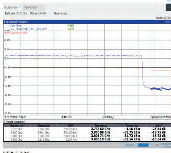
1-N78-3700-3800--30-70-H-3-DFT-PI2BPSK-Outer_Full-180@0-Ant1-PASS-see graph
