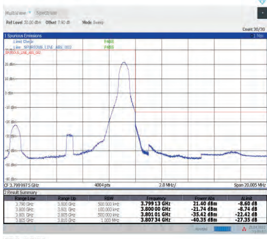
1-N78-3700-3800--30-10-H-5-CP-QPSK-Edge_1RB_R ight-1@23-Ant1-PASS-see graph
