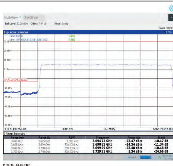
1-N78-3700-3800--30-40-L-6-CP-QPSK-Outer_Ful_I-106@0-Ant1-PASS-see graph
