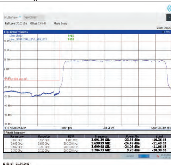
1-N78-3700-3800--30-20-L-3-DFT-PI2BPSK-Outer_Full-50@0-Ant1-PASS-see graph
