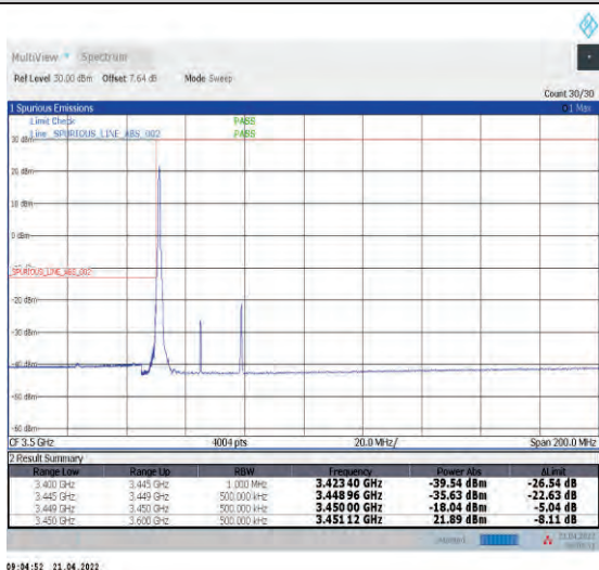
1-N78-3450-3550--30-30-L-4-CP-QPSK-Edge_1RB_L_eff-1@0-Ant1-PASS-see graph
