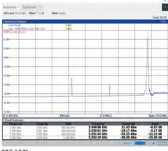
1-N78-3450-3550--30-80-H-2-DFT-PI2BPSK-Edge_1R_B_Right-1@216-Ant1-PASS-see graph
