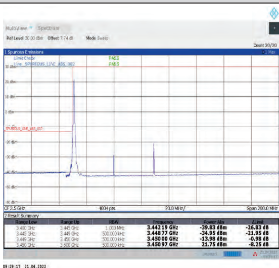
1-N78-3450-3550--30-60-L-4-CP-QPSK-Edge_1RB_L_eff-1@0-Ant1-PASS-see graph
