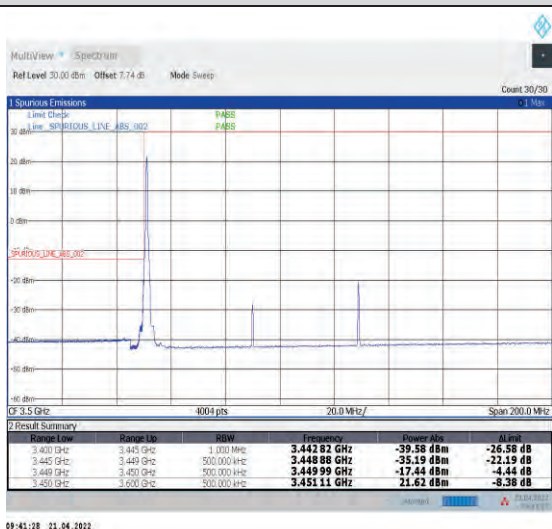
1-N78-3450-3550--30-80-L-4-CP-QPSK-Edge_1RB_L_eff-1@0-Ant1-PASS-see graph
