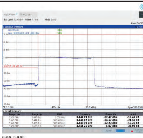
1-N78-3450-3550--30-80-L-6-CP-QPSK-Outer_Full-217@0-Ant1-PASS-see graph
