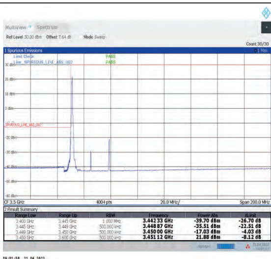
1-N78-3450-3550--30-30-L-1-DFT-PI2BPSK-Edge_1R_B_Left-1@0-Ant1-PASS-see graph
