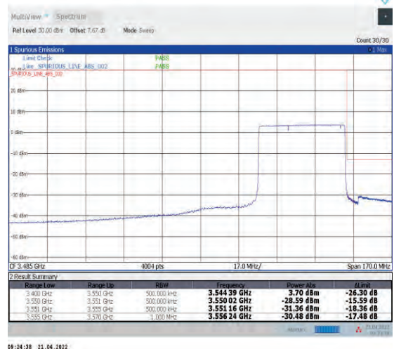
1-N78-3450-3550--30-40-H-6-CP-QPSK-Outer_Full-106@0-Ant1-PASS-see graph
