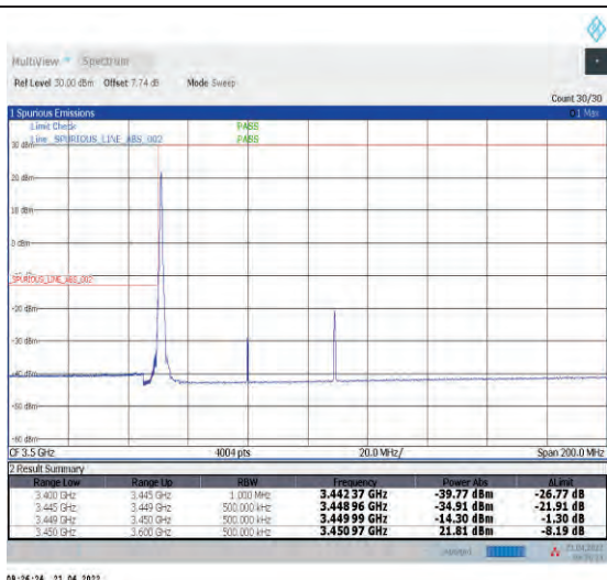
1-N78-3450-3550--30-60-L-1-DFT-PI2BPSK-Edge_1R_B_Left-1@0-Ant1-PASS-see graph
