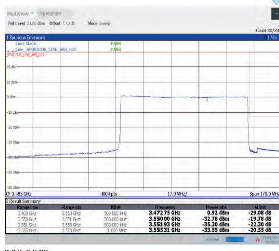
1-N78-3450-3550--30-80-H-6-CP-QPSK-Outer_Full-217@0-Ant1-PASS-see graph
