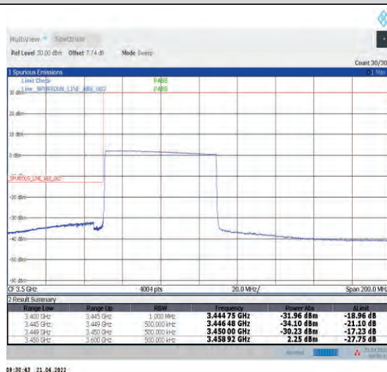
1-N78-3450-3550--30-60-L-6-CP-QPSK-Outer_Ful_I-162@0-Ant1-PASS-see graph
