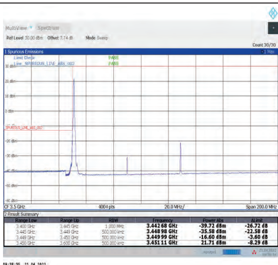
1-N78-3450-3550--30-80-L-1-DFT-PI2BPSK-Edge_1R_B_Left-1@0-Ant1-PASS-see graph
