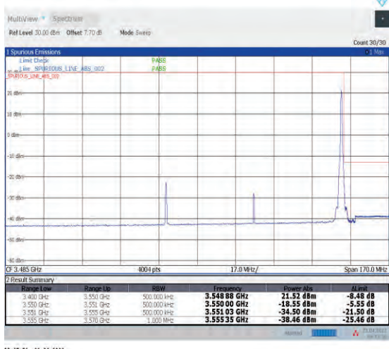
1-N78-3450-3550--30-80-H-5-CP-QPSK-Edge_1RB_Right-1@216-Ant1-PASS-see graph
