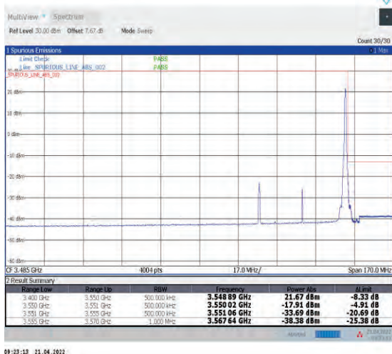
1-N78-3450-3550--30-40-H-5-CP-QPSK-Edge_1RB_Right-1@105-Ant1-PASS-see graph
