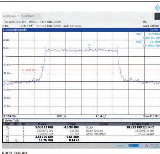
1-N78-3450-3550--30-20-H-9-CP-256QAM-Outer_Fu II-51@0-Ant1-18.223-19.760-≤20-PASS
