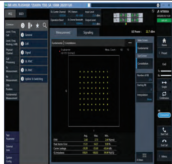
1-N78-3450-3550-PC1-30-100-M-8-CP-64QAM-Outer_Full-273@0-Ant1-see graph-PASS
