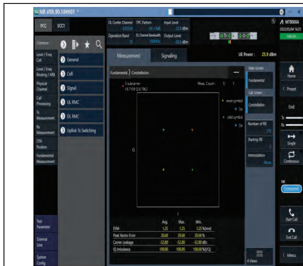
1-N78-3450-3550--30-100-M-1-DFT-PI2BPSK-Outter_Full-270@0-Ant1-see graph-PASS
