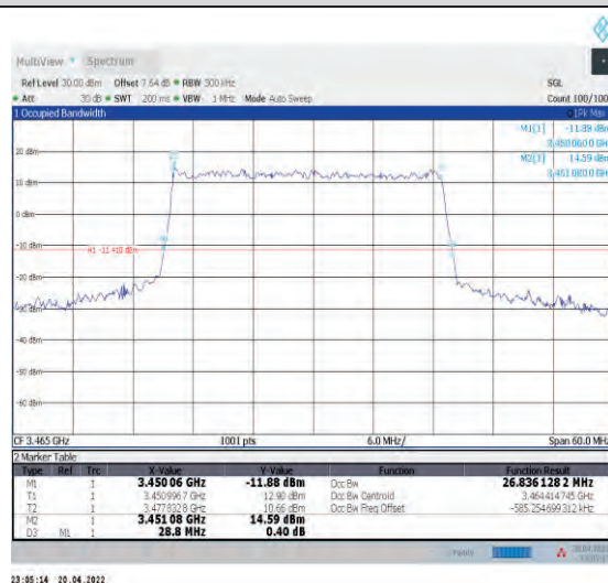
1-N78-3450-3550--30-30-L-3-DFT-16QAM-Outer_Fu ll-75@0-Ant1-26.836-28.800-≤30-PASS
