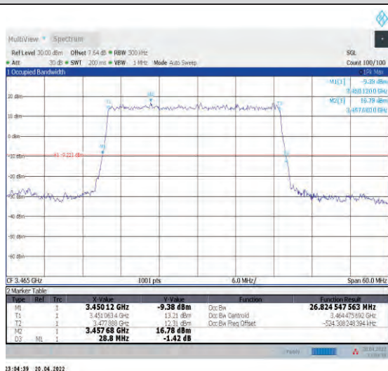
1-N78-3450-3550--30-30-L-2-DFT-PI2BPSK-Outer_F ull-75@0-Ant1-26.825-28.800-≤30-PASS
