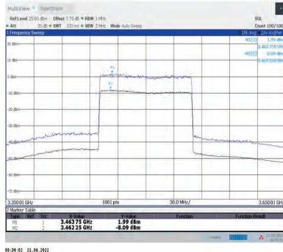
1-N78-3450-3550--30-100-M-2-CP-256QAM-Outer_Full-273@0-Ant1-10.08-100%-0.00-10.08-PASS-≤13
