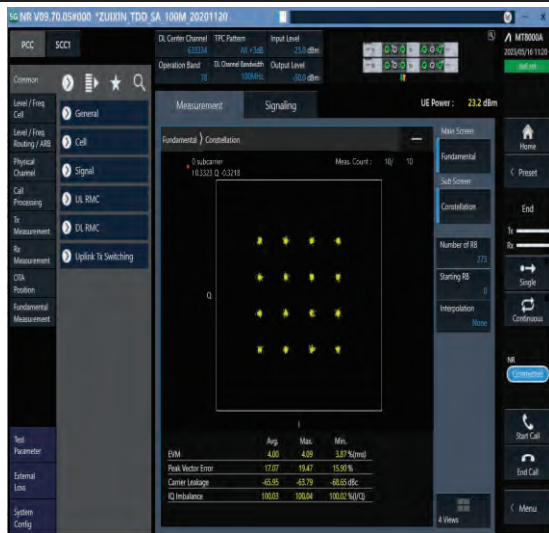
1-N78-3450-3550-PC1-30-100-M-7-CP-16QAM-Outer_Full-273@0-Ant1-see graph-PASS
