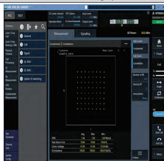
1-N78-3450-3550--30-100-M-4-DFT-64QAM-Outter_Full-270@0-Ant1-see graph-PASS
