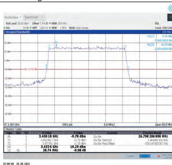
1-N78-3450-3550--30-30-L-1-DFT-QPSK-Outer_Full- 75@0-Ant1-26.798-28.740-≤30-PASS
