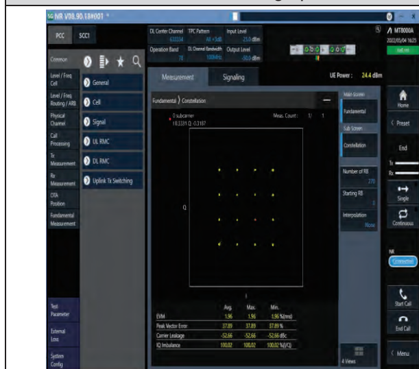
1-N78-3450-3550--30-100-M-3-DFT-16QAM-Outter_Full-270@0-Ant1-see graph-PASS
