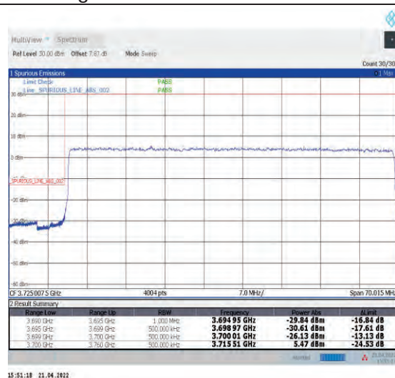
1-N77-3700-3980--30-60-L-3-DFT-PI2BPSK-Outer_Full-162@0-Ant1-PASS-see graph
