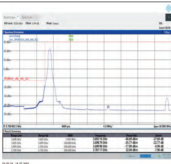
1-N77-3700-3980-PC1-30-30-L-1-DFT-PI2BPSK-Edge_1RB_Left-1@0-Ant1-1--PASS-see graph
