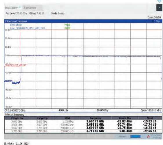
1-N77-3700-3980--30-90-L-6-CP-QPSK-Outer_Ful_I-245@0-Ant1-PASS-see graph
