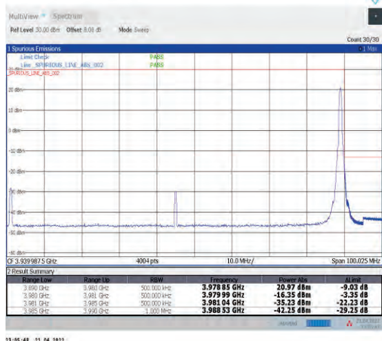
1-N77-3700-3980--30-90-H-2-DFT-PI2BPSK-Edge_1R B_Right-1@244-Ant1-PASS-see graph
