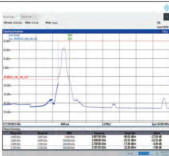
1-N77-3700-3980-PC1-30-20-L-1-DFT-PI2BPSK-Edg_e_1RB_Left-1@0-Ant1-1--PASS-see graph
