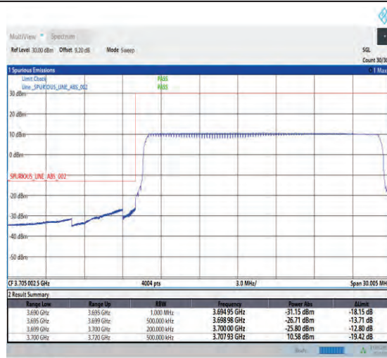
1-N77-3700-3980-PC1-30-20-L-3-DFT-PI2BPSK-Outer_Full-50@0-Ant1-1--PASS-see graph
