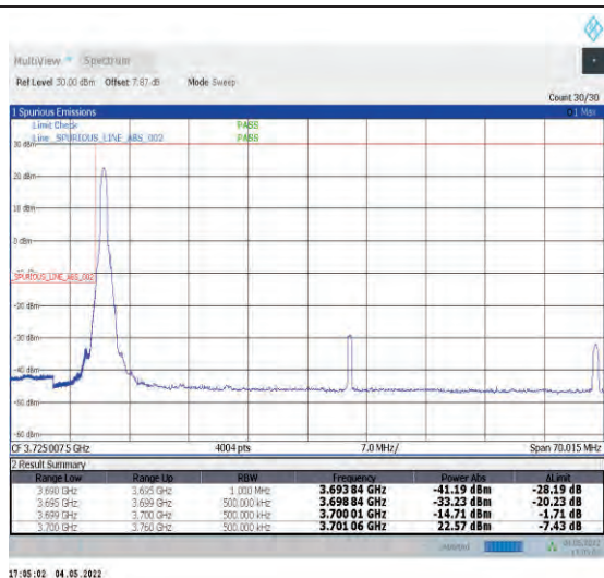
1-N77-3700-3980--30-60-L-1-DFT-PI2BPSK-Edge_1R_B_Left-1@0-Ant1-PASS-see graph
