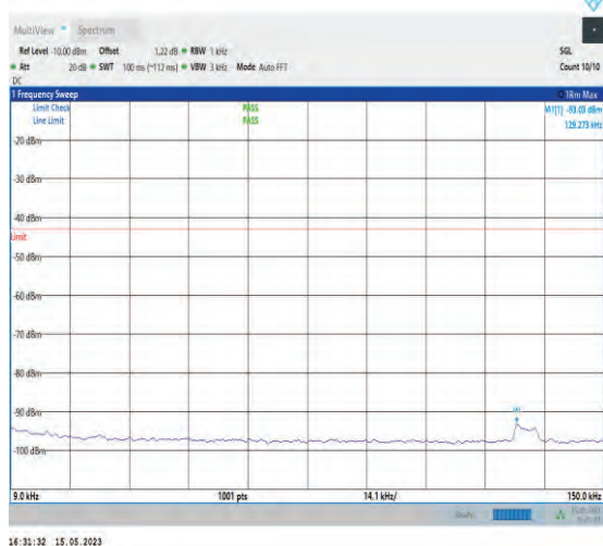
1-N77-3700-3980-PC1-30-100-L-1-DFT-PI2BPSK-In ner_1RB_Left-1@1-0.009-0.15-Ant1-0.13--93.03--4 3-PASS
