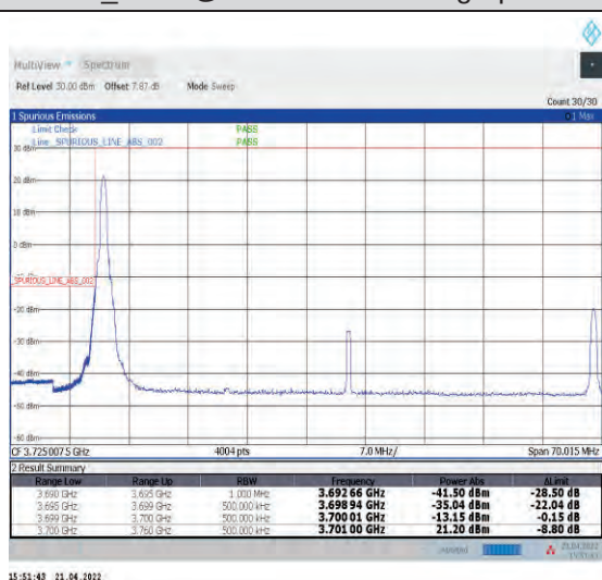
1-N77-3700-3980--30-60-L-4-CP-QPSK-Edge_1RB_L_eff-1@0-Ant1-PASS-see graph
