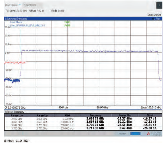
1-N77-3700-3980--30-90-L-3-DFT-PI2BPSK-Outer_Full-240@0-Ant1-PASS-see graph
