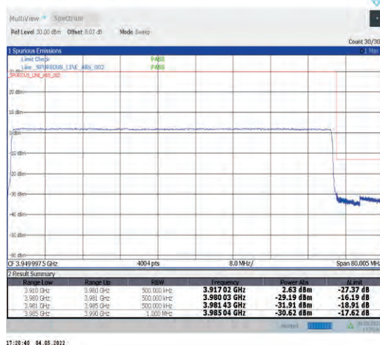
1-N77-3700-3980--30-70-H-6-CP-QPSK-Outer_Fu ll-189@0-Ant1-PASS-see graph
