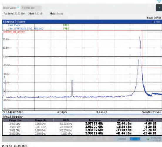
1-N77-3700-3980--30-70-H-5-CP-QPSK-Edge_1RB_R ight-1@188-Ant1-PASS-see graph
