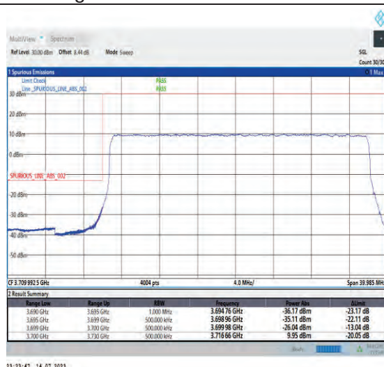
1-N77-3700-3980-PC1-30-30-L-3-DFT-PI2BPSK-Outer_Full-75@0-Ant1-1--PASS-see graph
