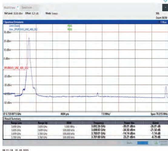
1-N77-3700-3980-PC1-30-60-L-4-CP-QPSK-Edge_1RB_Left-1@0-Ant1-1--PASS-see graph
