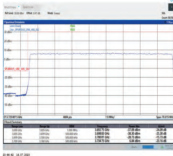
1-N77-3700-3980-PC1-30-60-L-3-DFT-PI2BPSK-Outer_Full-162@0-Ant1-1--PASS-see graph
