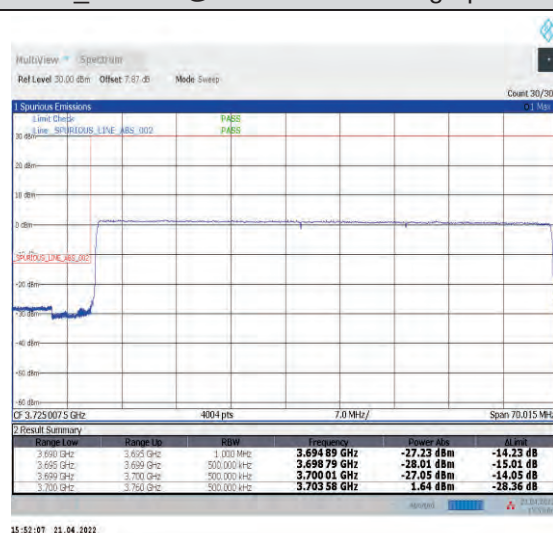
1-N77-3700-3980--30-60-L-6-CP-QPSK-Outer_Ful_I-162@0-Ant1-PASS-see graph
