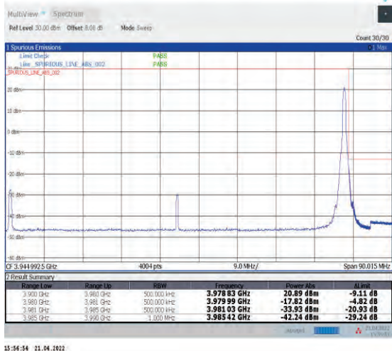
1-N77-3700-3980--30-80-H-2-DFT-PI2BPSK-Edge_1R_B_Right-1@216-Ant1-PASS-see graph
