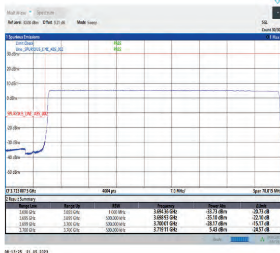
1-N77-3700-3980-PC1-30-60-L-6-CP-QPSK-Outer_Full-162@0-Ant1-1--PASS-see graph
