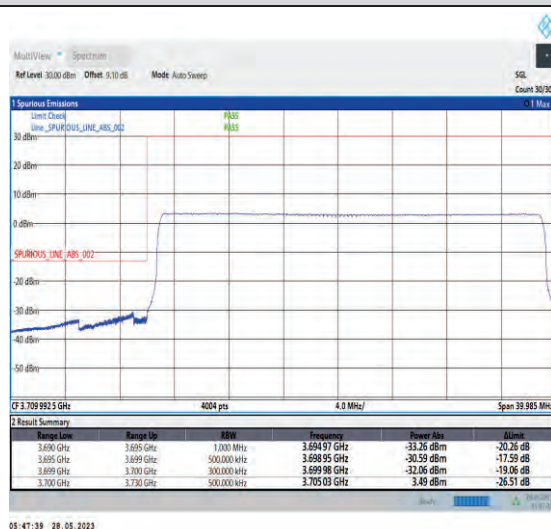
1-N77-3700-3980-PC1-30-30-L-6-CP-QPSK-Outer_Full-78@0-Ant1-1--PASS-see graph
