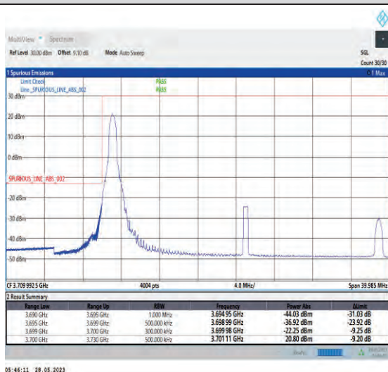
1-N77-3700-3980-PC1-30-30-L-4-CP-QPSK-Edge_1RB_Left-1@0-Ant1-1--PASS-see graph
