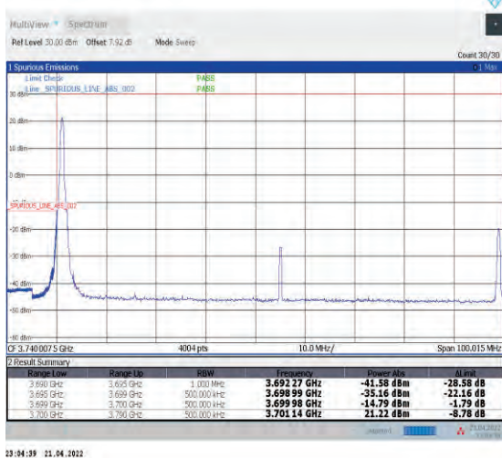
1-N77-3700-3980--30-90-L-4-CP-QPSK-Edge_1RB_L_eff-1@0-Ant1-PASS-see graph
