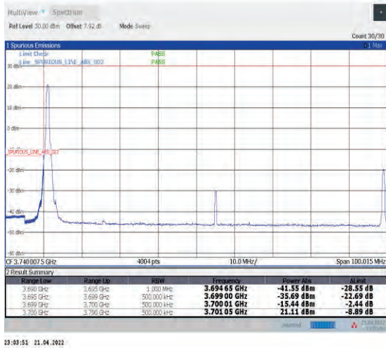
1-N77-3700-3980--30-90-L-1-DFT-PI2BPSK-Edge_1R_B_Left-1@0-Ant1-PASS-see graph
