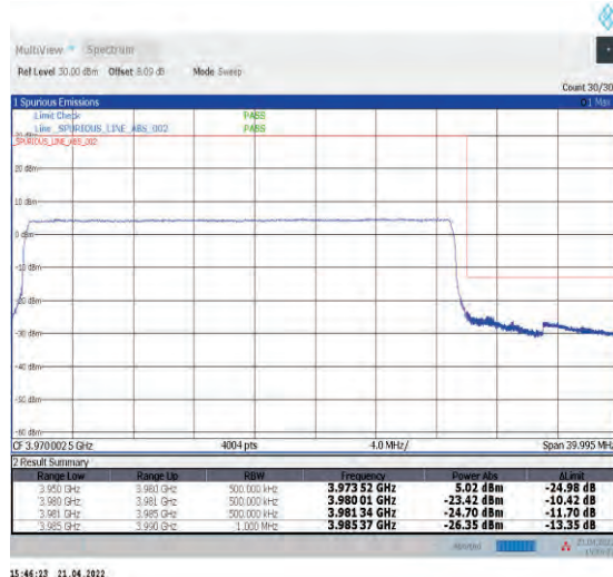
1-N77-3700-3980--30-30-H-6-CP-QPSK-Outer_Fu ll-78@0-Ant1-PASS-see graph
