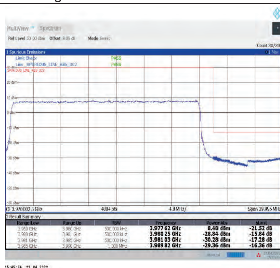
1-N77-3700-3980--30-30-H-3-DFT-PI2BPSK-Outer _Full-75@0-Ant1-PASS-see graph
