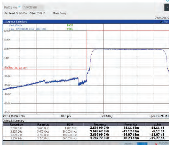
1-N77-3700-3980--30-10-L-6-CP-QPSK-Outer_Ful l-24@0-Ant1-PASS-see graph
