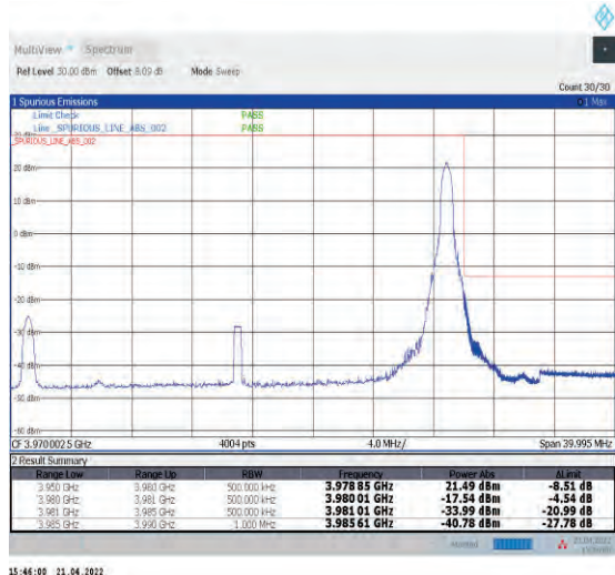
1-N77-3700-3980--30-30-H-5-CP-QPSK-Edge_1RB_R ight-1@77-Ant1-PASS-see graph
