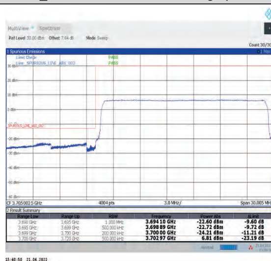
1-N77-3700-3980--30-20-L-6-CP-QPSK-Outer_Ful l-51@0-Ant1-PASS-see graph
