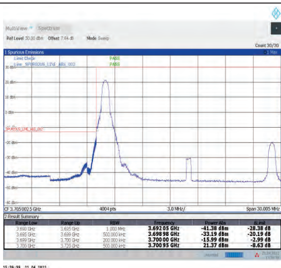
1-N77-3700-3980--30-20-L-1-DFT-PI2BPSK-Edge_1R_B_Left-1@0-Ant1-PASS-see graph
