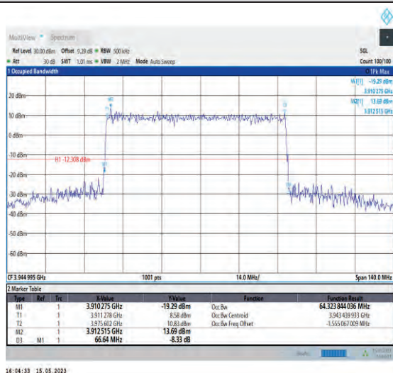
1-N77-3700-3980-PC1-30-70-H-4-DFT-64QAM-Out er_Full-180@0-Ant1-64.324-66.640-≤70-PASS
