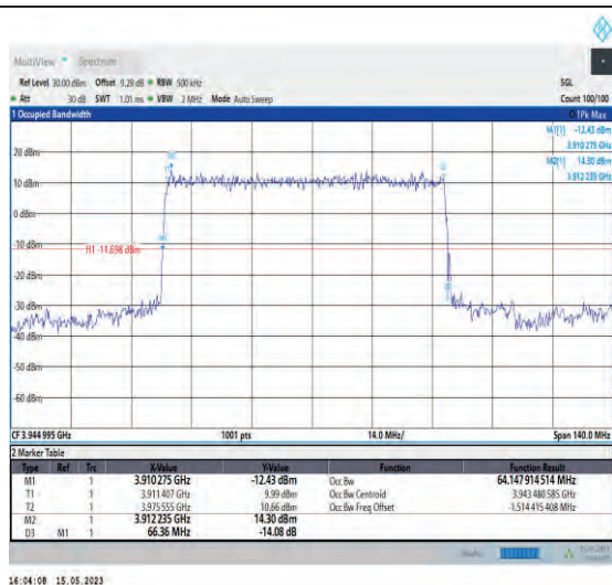
1-N77-3700-3980-PC1-30-70-H-2-DFT-PI2BPSK-Out er_Full-180@0-Ant1-64.148-66.360-≤70-PASS
