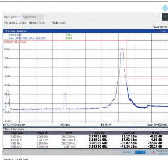
1-N77-3700-3980--30-30-H-2-DFT-PI2BPSK-Edge_1R B_Right-1@77-Ant1-PASS-see graph
