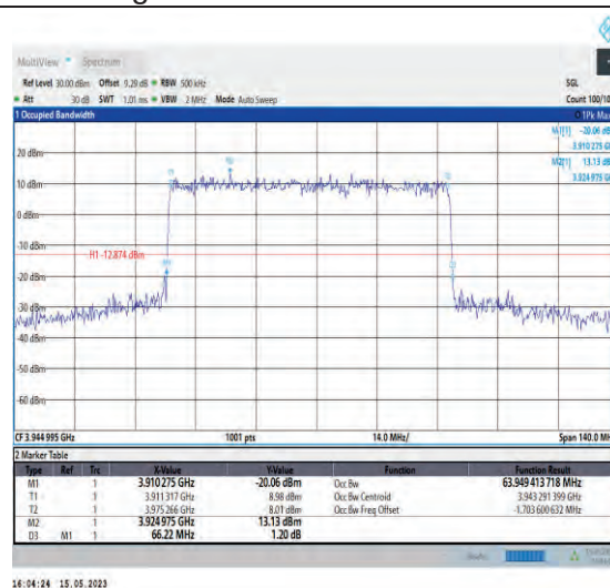
1-N77-3700-3980-PC1-30-70-H-3-DFT-16QAM-Out er_Full-180@0-Ant1-63.949-66.220-≤70-PASS
