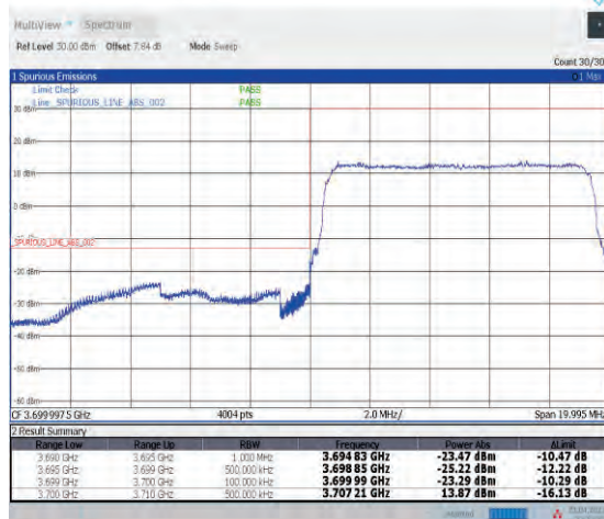
1-N77-3700-3980--30-10-L-3-DFT-PI2BPSK-Outer _Full-24@0-Ant1-PASS-see graph
