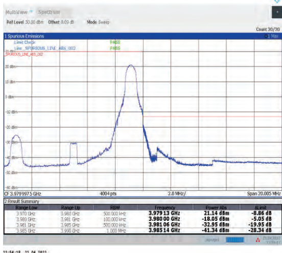
1-N77-3700-3980--30-10-H-2-DFT-PI2BPSK-Edge_1R B_Right-1@23-Ant1-PASS-see graph
