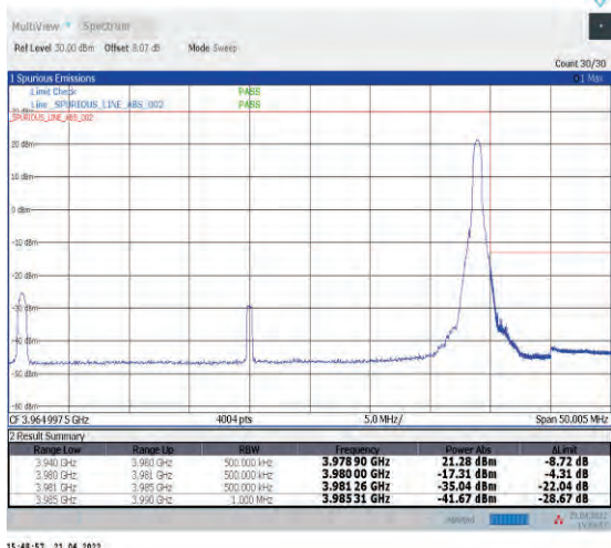
1-N77-3700-3980--30-40-H-2-DFT-PI2BPSK-Edge_1R B_Right-1@105-Ant1-PASS-see graph
