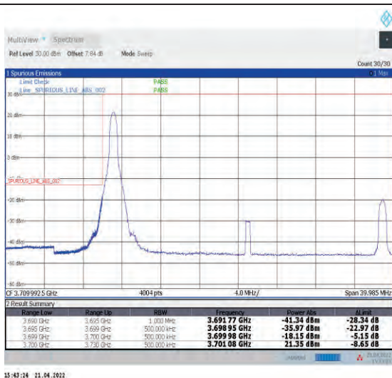
1-N77-3700-3980--30-30-L-1-DFT-PI2BPSK-Edge_1R B_Left-1@0-Ant1-PASS-see graph
