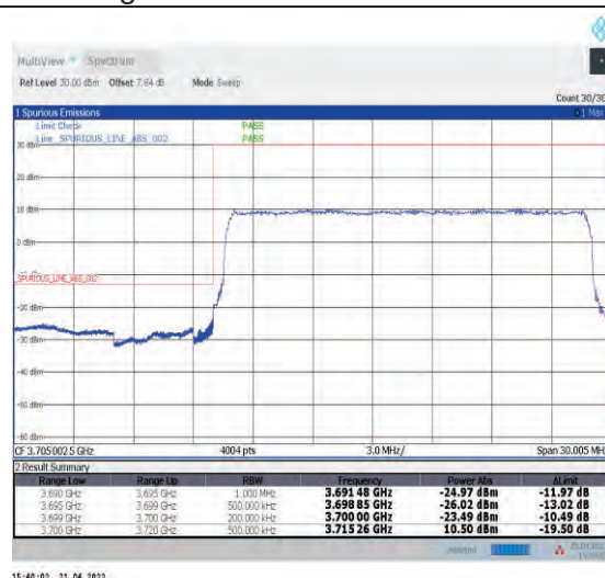
1-N77-3700-3980--30-20-L-3-DFT-PI2BPSK-Outer_Full-50@0-Ant1-PASS-see graph
