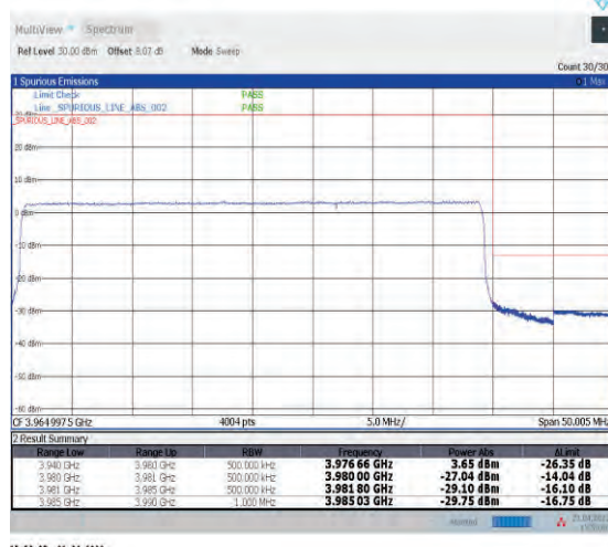
1-N77-3700-3980--30-40-H-6-CP-QPSK-Outer_Fu ll-106@0-Ant1-PASS-see graph
