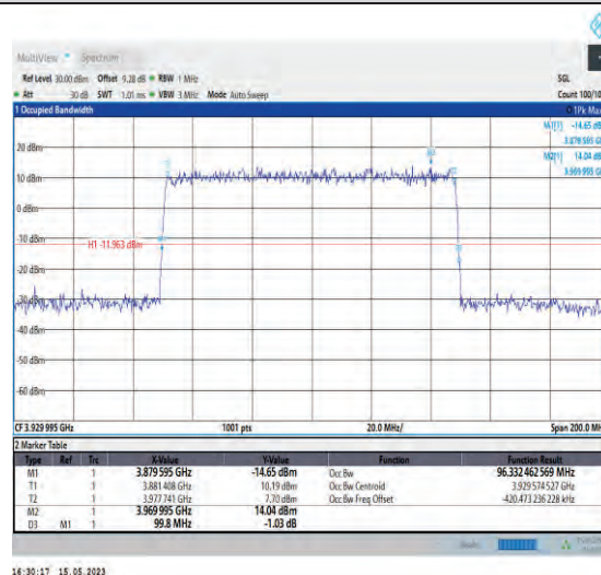
1-N77-3700-3980-PC1-30-100-H-4-DFT-64QAM-Ou ter_Full-270@0-Ant1-96.332-99.800-≤100-PASS
