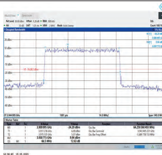
1-N77-3700-3980-PC1-30-70-H-5-DFT-256QAM-Out er_Full-180@0-Ant1-64.259-66.500-≤70-PASS
