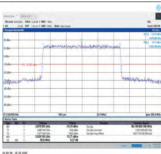
1-N77-3700-3980-PC1-30-100-H-1-DFT-QPSK-Outer_Full-270@0-Ant1-96.195-99.800-≤100-PASS
