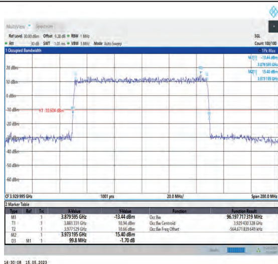
1-N77-3700-3980-PC1-30-100-H-3-DFT-16QAM-Out er_Full-270@0-Ant1-96.198-99.800-≤100-PASS
