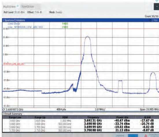
1-N77-3700-3980--30-10-L-1-DFT-PI2BPSK-Edge_1R B_Left-1@0-Ant1-PASS-see graph
