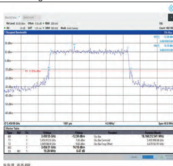
1-N78-3450-3550-PC1-30-20-L-8-CP-64QAM-Outer_Full-51@0-Ant1-18.168-19.280-≤20-PASS
