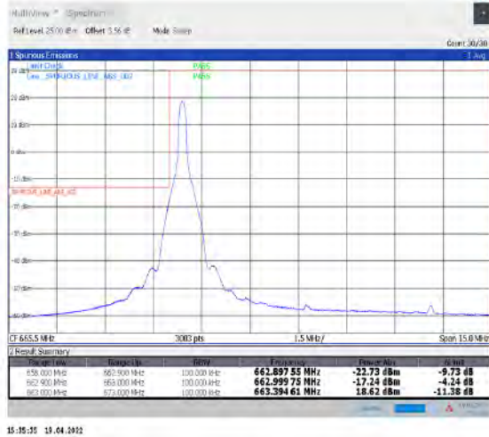
1-N71--15-10-L-1-DFT-PI2BPSK-Edge_1RB_Left-1@0-Ant1-PASS-see graph
