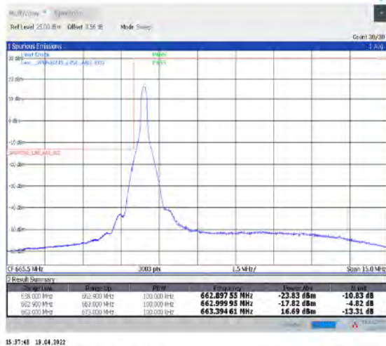
1-N71--15-10-L-4-CP-QPSK-Edge_1RB_Left-1@0-Ant1-PASS-see graph
