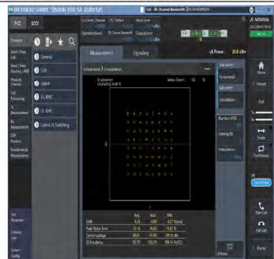
1-N71--15-20-M-8-CP-64QAM-Outer_Full-106@0-Ant1-see graph-PASS
