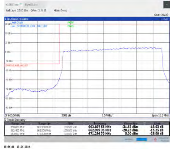
1-N71--15-10-L-3-DFT-PI2BPSK-Outer_Full-50@0-Ant1-PASS-see graph
