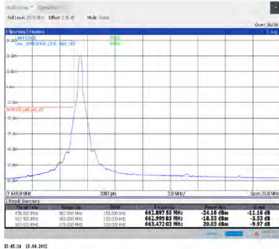
1-N71--15-15-L-1-DFT-PI2BPSK-Edge_1RB_Left-1@0-Ant1-PASS-see graph
