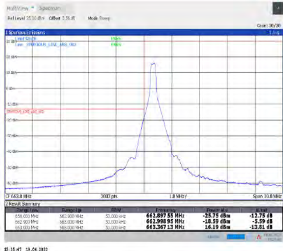
1-N71--15-5-L-1-DFT-PI2BPSK-Edge_1RB_Left-1@0-Ant1-PASS-see graph
