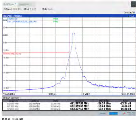
1-N71--15-5-L-4-CP-QPSK-Edge_1RB_Left-1@0-Ant1-PASS-see graph
