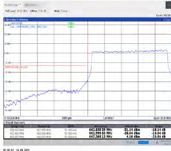
1-N71--15-5-L-3-DFT-PI2BPSK-Outer_Full-25@0-Ant1-PASS-see graph
