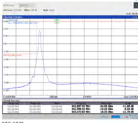
1-N71--15-15-L-4-CP-QPSK-Edge_1RB_Left-1@0-Ant1-PASS-see graph
