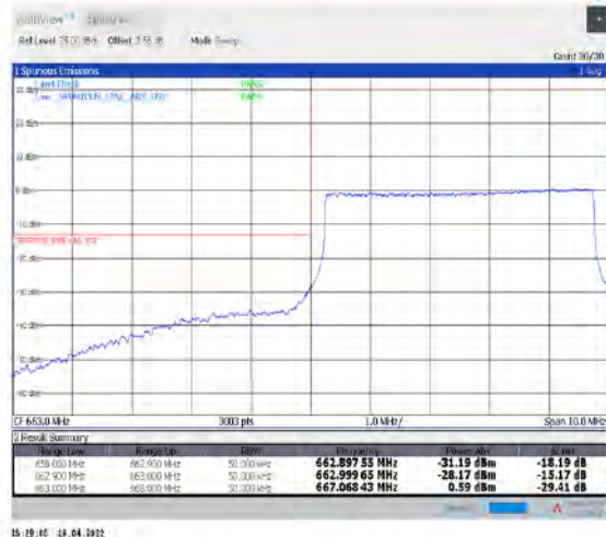
1-N71--15-5-L-6-CP-QPSK-Outer_Full-25@0-Ant1-PASS-see graph
