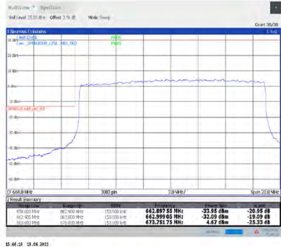
1-N71--15-15-L-3-DFT-PI2BPSK-Outer_Full-75@0-Ant1-PASS-see graph
