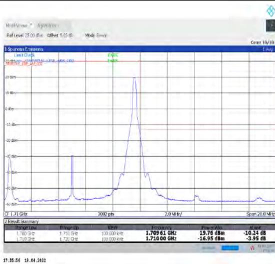
1-N70-15-10-H-2-DFT-PI2BPSK-Edge_1RB_Right-1@51-Ant1-seegraph-PASS-see graph
