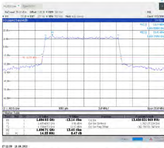
1-N70--15-15-H-3-DFT-16QAM-Outer_Full-75@0-Ant1-13.456-14.550-≤15-PASS
