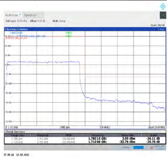
1-N70-15-10-H-3-DFT-PI2BPSK-Outer_Full-50@0-Ant1-seegraph-PASS-see graph
