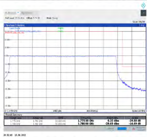
1-N66-PC3-15-5-H-6-CP-QPSK-Outer_Full-25@0-Ant1-seegraph-PASS-see graph
