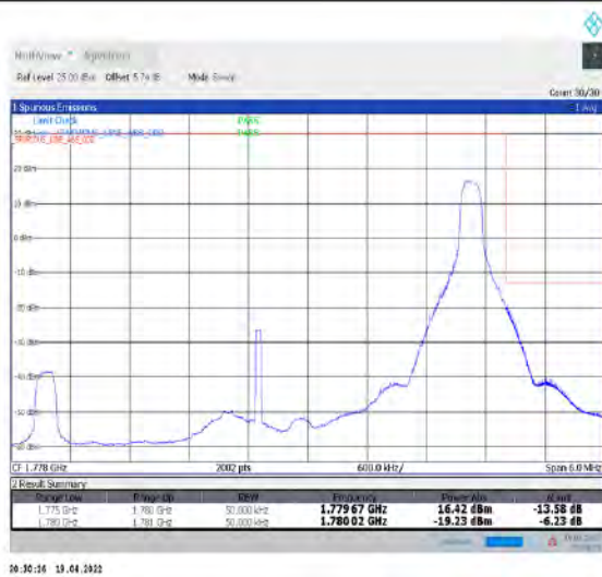
1-N66-PC3-15-5-H-2-DFT-PI2BPSK-Edge_1RB_Right-1@24-Ant1-seegraph-PASS-see graph
