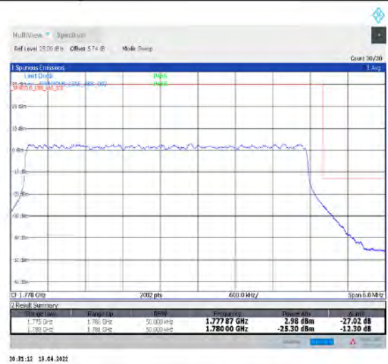
1-N66-PC3-15-5-H-3-DFT-PI2BPSK-Outer_Full-25@0-Ant1-seegraph-PASS-see graph
