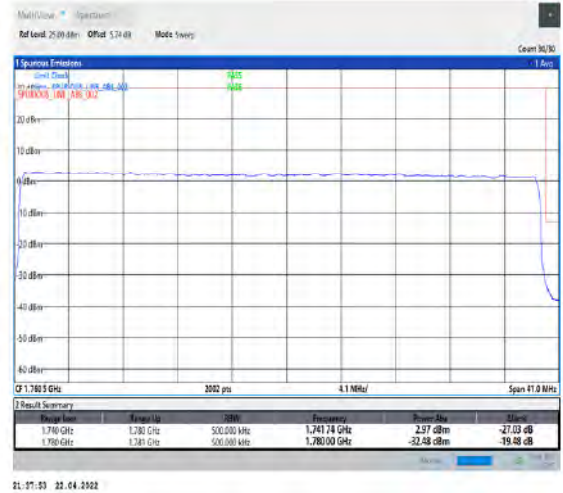
1-N66-PC3-15-40-H-3-DFT-PI2BPSK-Outer_Full-216@0-Ant1-seegraph-PASS-see graph
