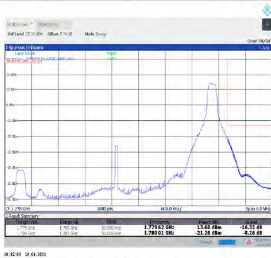
1-N66-PC3-15-5-H-5-CP-QPSK-Edge_1RB_Right-1@24-Ant1-seegraph-PASS-see graph
