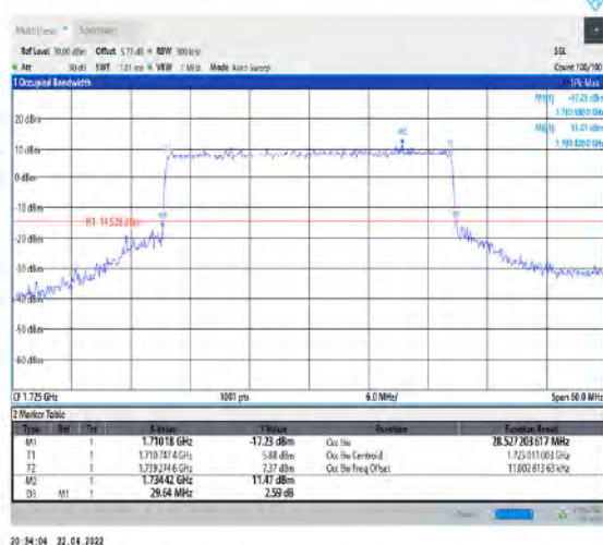
1-N66-PC3-15-30-L-8-CP-64QAM-Outer_Full-160@0-Ant1-28.527-29.640-≤30-PASS
