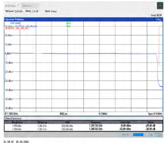
1-N66-PC3-15-40-H-6-CP-QPSK-Outer_Full-216@0-Ant1-seegraph-PASS-see graph
