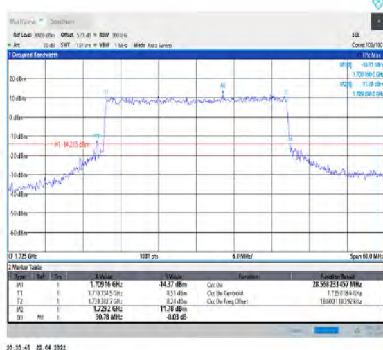
1-N66-PC3-15-30-L-6-CP-QPSK-Outer_Full-160@0-Ant1-28.568-30.780-≤30-PASS
