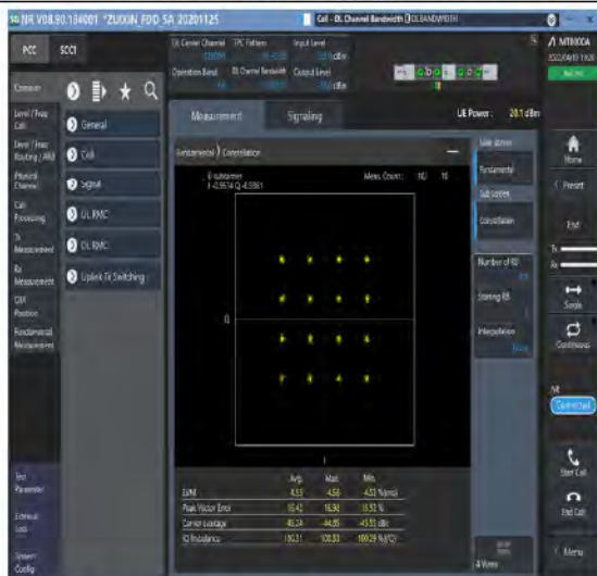
1-N66-PC3-15-20-M-7-CP-16QAM-Outer_Full-106@0-Ant1-see graph-PASS
