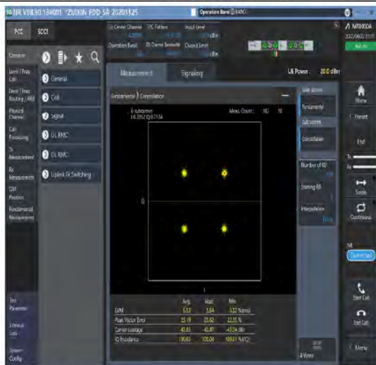
1-N66-PC3-15-40-M-6-CP-QPSK-Outer_Full-216@0-Ant1-see graph-PASS
