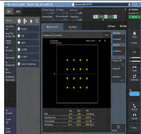
1-N66-PC3-15-40-M-7-CP-16QAM-Outer_Full-216@0-Ant1-see graph-PASS
