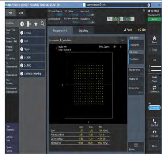
1-N66-PC3-15-40-M-5-DFT-256QAM-Outer_Full-216@0-Ant1-see graph-PASS
