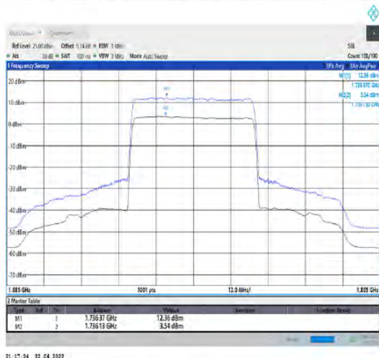
1-N66-PC3-15-40-M-1-DFT-256QAM-Outer_Full-216@0-Ant1-8.82-100%-0.00-8.82-PASS-≤13
