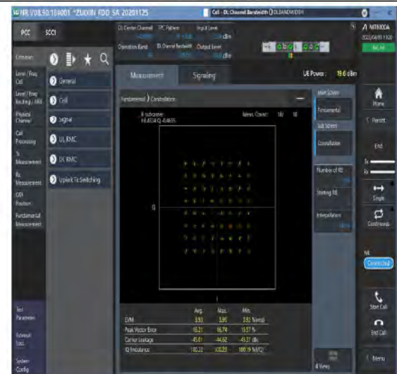
1-N66-PC3-15-20-M-8-CP-64QAM-Outer_Full-106@0-Ant1-see graph-PASS
