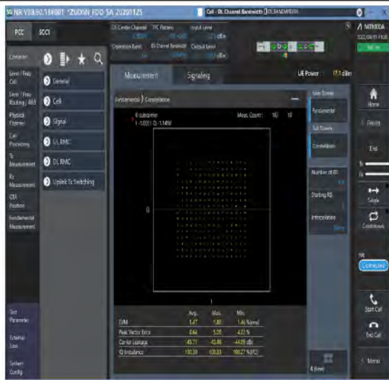
1-N66-PC3-15-20-M-9-CP-256QAM-Outer_Full-106@0-Ant1-see graph-PASS
