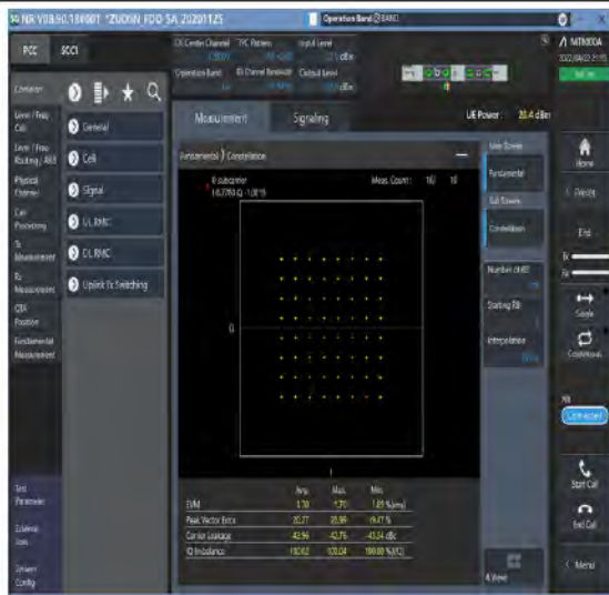
1-N66-PC3-15-40-M-4-DFT-64QAM-Outer_Full-216@0-Ant1-see graph-PASS
