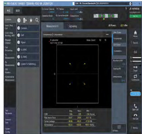
1-N66-PC3-15-20-M-2-DFT-QPSK-Outer_Full-100@0-Ant1-see graph-PASS
