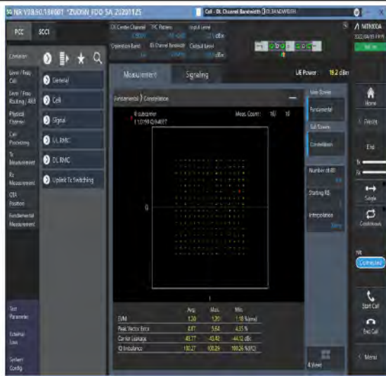
1-N66-PC3-15-20-M-5-DFT-256QAM-Outer_Full-100@0-Ant1-see graph-PASS
