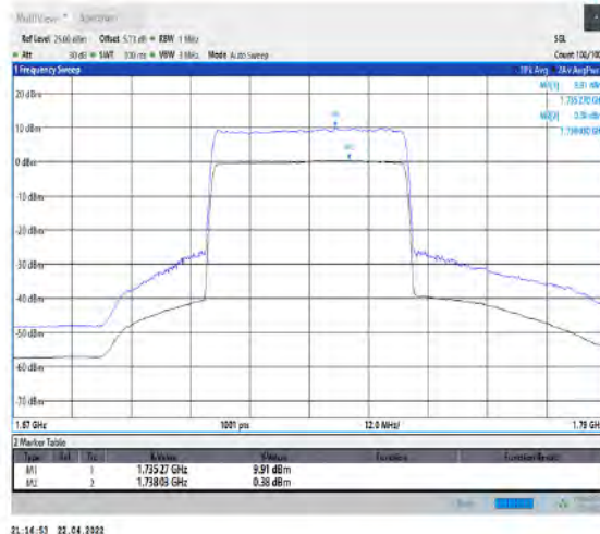
1-N66-PC3-15-40-L-2-CP-256QAM-Outer_Full-216@0-Ant1-9.53-100%-0.00-9.53-PASS-≤13
