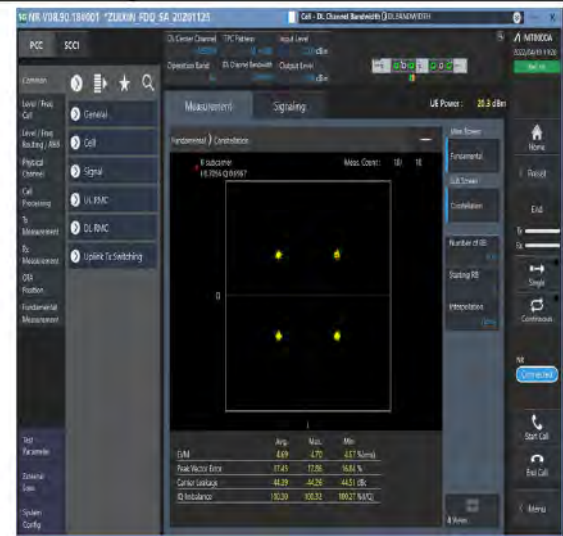
1-N66-PC3-15-20-M-6-CP-QPSK-Outer_Full-106@0-Ant1-see graph-PASS
