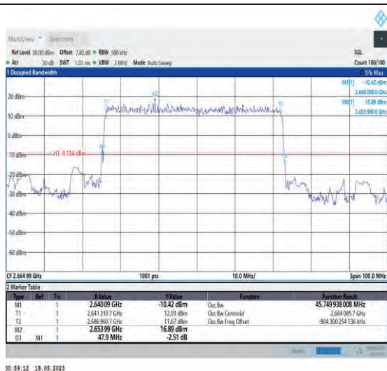
1-N41-PC1-30-50-H-2-DFT-PI2BPSK-Outter_Full-128 @0-Ant1-45.75-47.900-≤50-PASS
