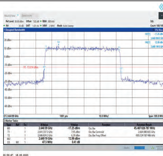
1-N41-PC1-30-50-H-5-DFT-256QAM-Outter_Full-128 @0-Ant1-45.487-47.500-≤50-PASS
