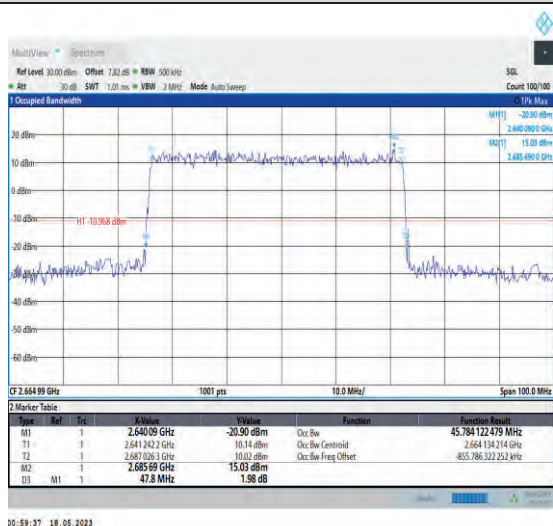
1-N41-PC1-30-50-H-4-DFT-64QAM-Outter_Full-128 @0-Ant1-45.784-47.800-≤50-PASS
