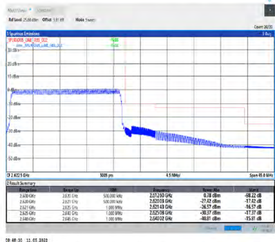
1-N38-PC2-30-20-H-6-CP-QPSK-Outer_Full-51@0-Ant1-PASS-see graph
