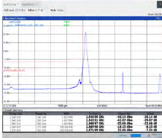
1-N38--30-30-L-1-DFT-PI2BPSK-Edge_1RB_Left-1@0-Ant1-PASS-see graph
