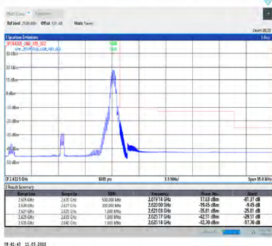
1-N38-PC2-30-15-H-5-CP-QPSK-Edge_1RB_Right- 1@37-Ant1-PASS-see graph
