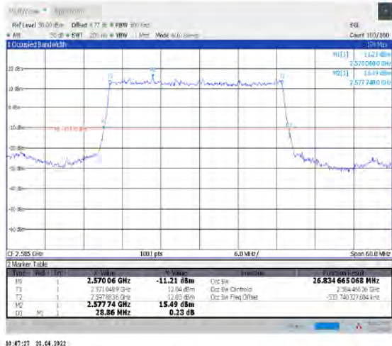
1-N38--30-30-L-2-DFT-PI2BPSK-Outer_Full-75@0- Ant1-26.835-28.860-≤30-PASS
