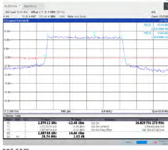
1-N38-30-30-L-1-DFT-QPSK-Outer_Full-75@0- Ant1-26.83-28.740-<30-PASS
