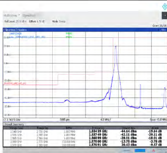
1-N38--30-15-L-1-DFT-PI2BPSK-Edge_1RB_Left-1@0-Ant1-PASS-see graph
