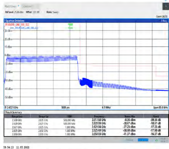
1-N38-PC2-30-30-H-6-CP-QPSK-Outer_Full-78@0-Ant1-PASS-see graph
