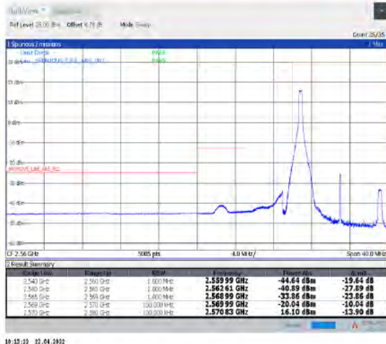
1-N38--30-10-L-4-CP-QPSK-Edge_1RB_Left-1@0-Ant1-PASS-see graph
