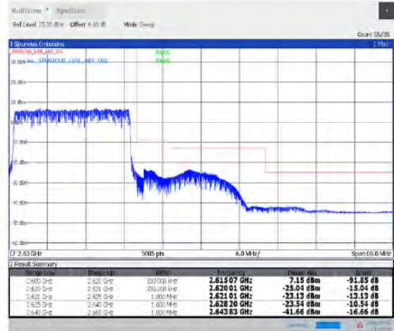
1-N38--30-20-H-3-DFT-PI2BPSK-Outer_Full-50@0-Ant1-PASS-see graph
