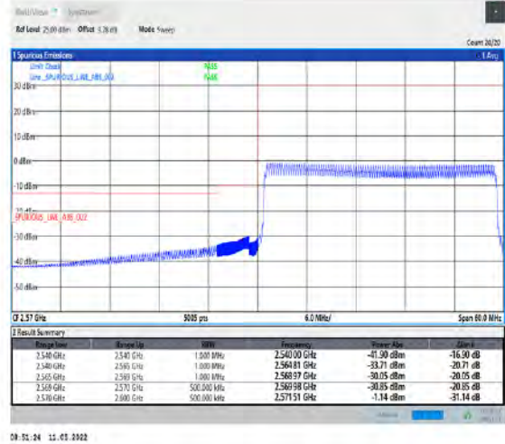
1-N38-PC2-30-30-L-6-CP-QPSK-Outer_Full-78@0-Ant1-PASS-see graph
