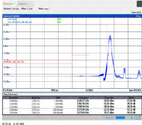
1-N38-PC2-30-10-L-4-CP-QPSK-Edge_1RB_Left-1@0-Ant1-PASS-see graph
