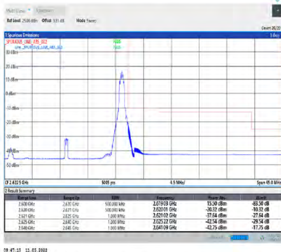
1-N38-PC2-30-20-H-5-CP-QPSK-Edge_1RB_Right-1@50-Ant1-PASS-see graph
