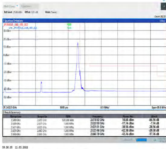
1-N38-PC2-30-40-H-5-CP-QPSK-Edge_1RB_Right-1@105-Ant1-PASS-see graph
