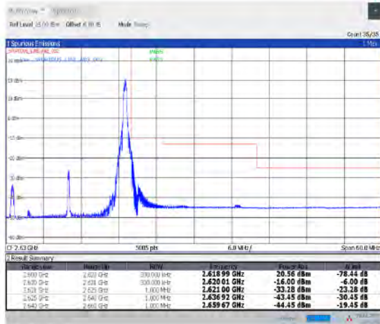
1-N38--30-20-H-5-CP-QPSK-Edge_1RB_Right-1@50-Ant1-PASS-see graph
