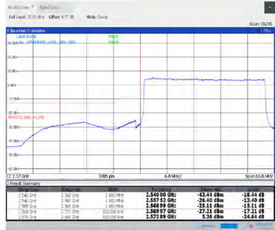
1-N38--30-30-L-3-DFT-PI2BPSK-Outer_Full-75@0-Ant1-PASS-see graph
