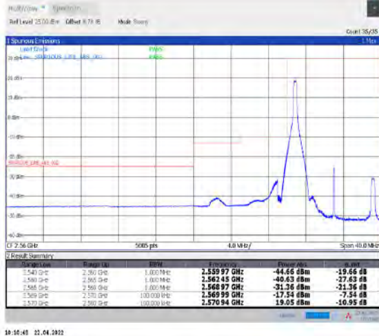
1-N38--30-10-L-1-DFT-PI2BPSK-Edge_1RB_Left-1@0-Ant1-PASS-see graph
