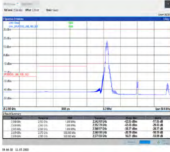
1-N38-PC2-30-20-L-4-CP-QPSK-Edge_1RB_Left-1@0-Ant1-PASS-see graph
