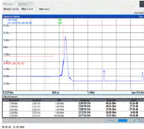
1-N38-PC2-30-40-L-4-CP-QPSK-Edge_1RB_Left-1@0-Ant1-PASS-see graph
