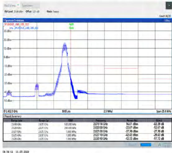
1-N38-PC2-30-10-H-5-CP-QPSK-Edge_1RB_Right-1@23-Ant1-PASS-see graph
