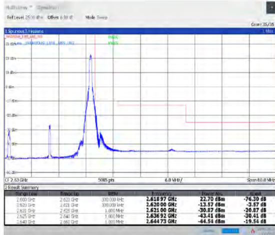
1-N38--30-20-H-2-DFT-PI2BPSK-Edge_1RB_Right-1@50-Ant1-PASS-see graph
