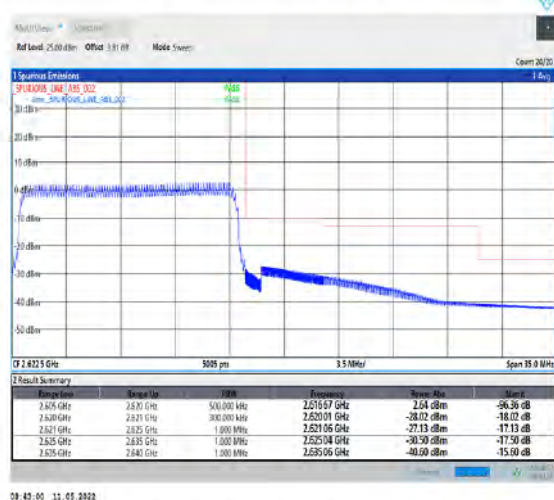
1-N38-PC2-30-15-H-6-CP-QPSK-Outer_Full- 38@0-Ant1-PASS-see graph
