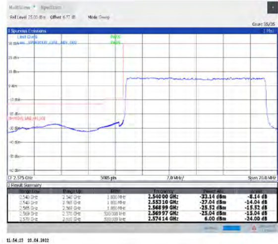
1-N38--30-40-L-3-DFT-PI2BPSK-Outer_Full-100@0-Ant1-PASS-see graph
