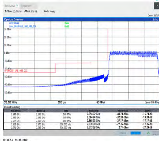
1-N38-PC2-30-15-L-6-CP-QPSK-Outer_Full- 38@0-Ant1-PASS-see graph
