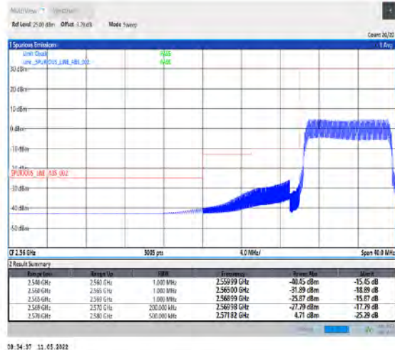
1-N38-PC2-30-10-L-6-CP-QPSK-Outer_Full-24@0-Ant1-PASS-see graph
