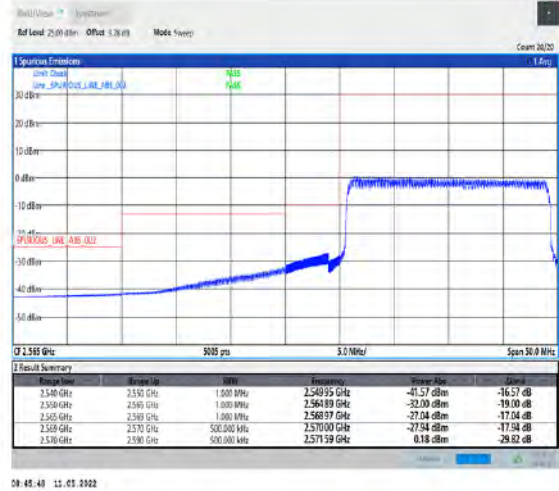
1-N38-PC2-30-20-L-6-CP-QPSK-Outer_Full-51@0-Ant1-PASS-see graph
