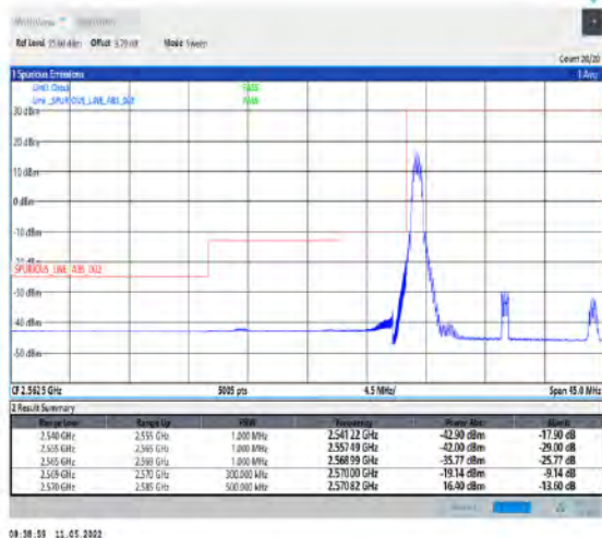
1-N38-PC2-30-15-L-4-CP-QPSK-Edge_1RB_Left- 1@0-Ant1-PASS-see graph
