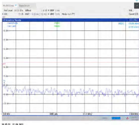
1-N38--30-40-L-1-DFT-PI2BPSK-Inner_1RB_Left- 1@1-0.009-0.15-Ant1--78.06--55-PASS
