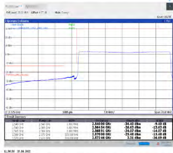
1-N38--30-40-L-6-CP-QPSK-Outer_Full-106@0-Ant1-PASS-see graph
