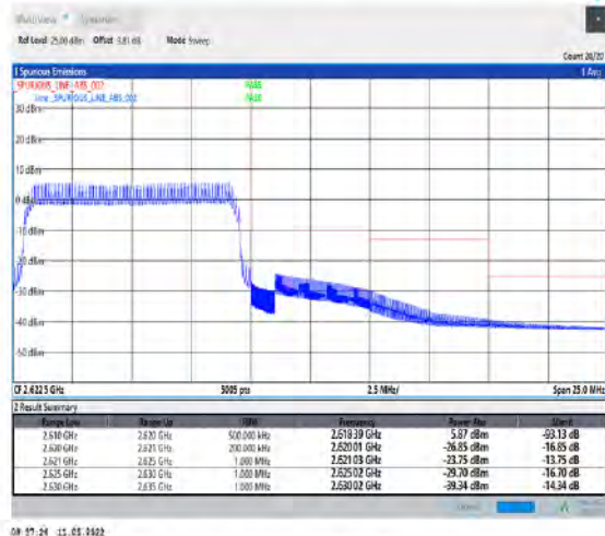
1-N38-PC2-30-10-H-6-CP-QPSK-Outer_Full-24@0-Ant1-PASS-see graph
