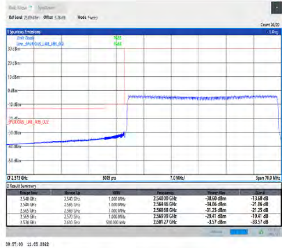
1-N38-PC2-30-40-L-6-CP-QPSK-Outer_Full-106@0-Ant1-PASS-see graph
