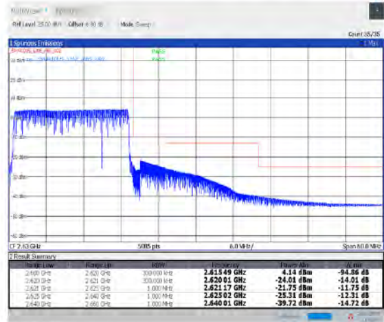
1-N38--30-20-H-6-CP-QPSK-Outer_Full-51@0-Ant1-PASS-see graph
