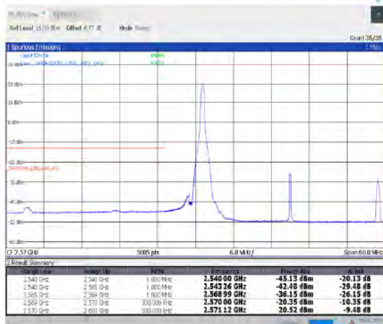
1-N38--30-30-L-4-CP-QPSK-Edge_1RB_Left-1@0-Ant1-PASS-see graph
