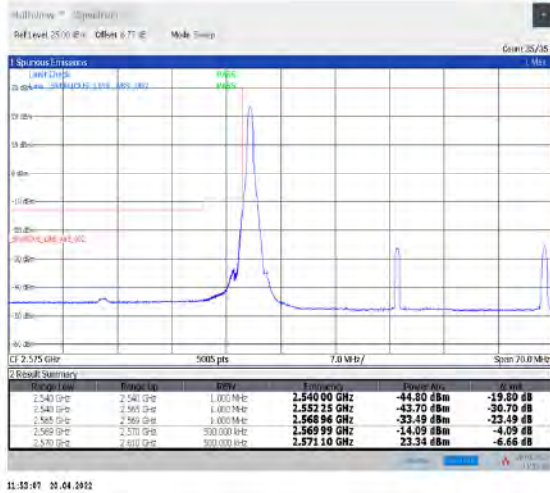
1-N38--30-40-L-1-DFT-PI2BPSK-Edge_1RB_Left-1@0-Ant1-PASS-see graph
