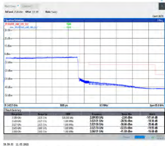
1-N38-PC2-30-40-H-6-CP-QPSK-Outer_Full-106@0-Ant1-PASS-see graph
