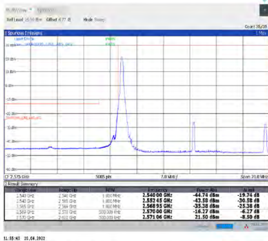
1-N38--30-40-L-4-CP-QPSK-Edge_1RB_Left-1@0-Ant1-PASS-see graph
