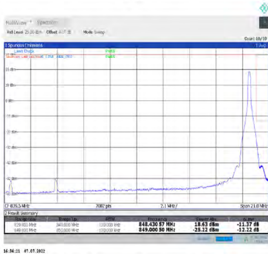
1-N26-824-849--15-20-H-5-CP-QPSK-Edge_1RB_Right-1@105-Ant1-seegraph-PASS-see graph
