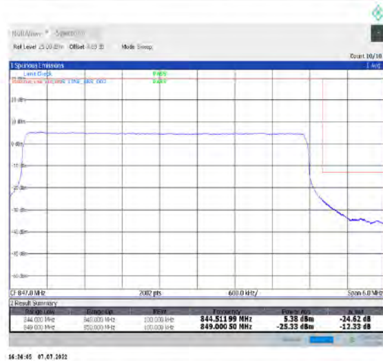
1-N26-824-849--15-5-H-6-CP-QPSK-Outer_Full-25@0-Ant1-seegraph-PASS-see graph
