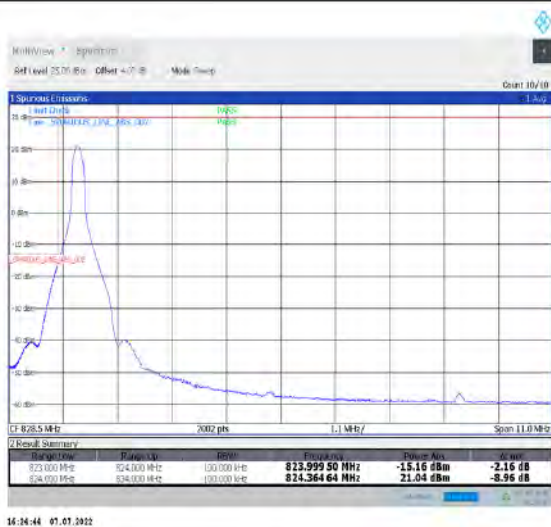
1-N26-824-849--15-10-L-1-DFT-PI2BPSK-Edge_1RB_Left-1@0-Ant1-seegraph-PASS-see graph
