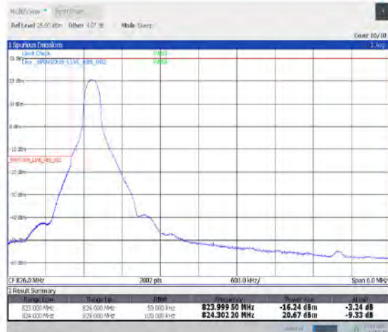
1-N26-824-849--15-5-L-1-DFT-PI2BPSK-Edge_1RB_Left-1@0-Ant1-seegraph-PASS-see graph
