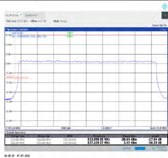
1-N26-824-849--15-15-L-3-DFT-PI2BPSK-Outer_Full-75@0-Ant1-seegraph-PASS-see graph
