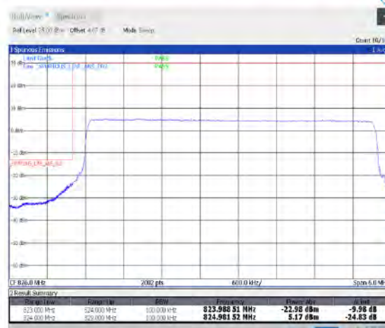
1-N26-824-849--15-5-L-6-CP-QPSK-Outer_Full-25@0-Ant1-seegraph-PASS-see graph
