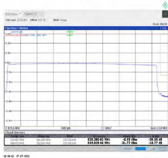
1-N26-824-849--15-20-H-3-DFT-PI2BPSK-Outer_Full-100@0-Ant1-seegraph-PASS-see graph
