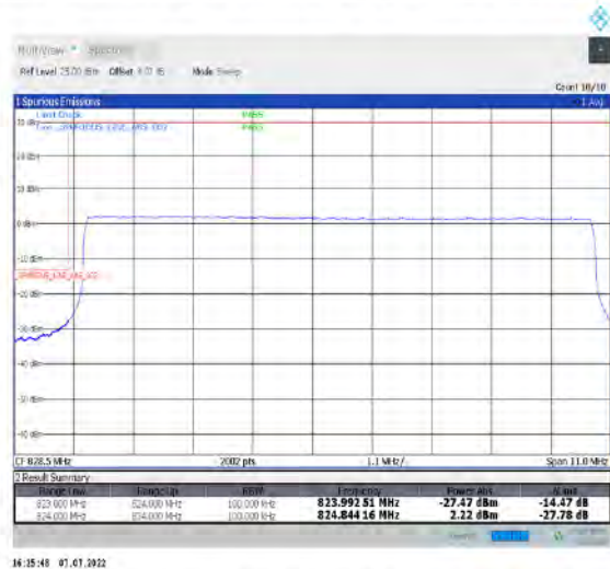
1-N26-824-849--15-10-L-6-CP-QPSK-Outer_Full-52@0-Ant1-seegraph-PASS-see graph
