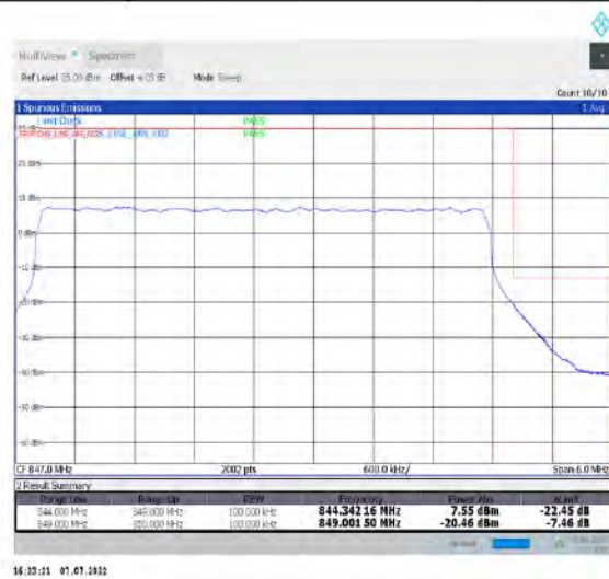
1-N26-824-849--15-5-H-3-DFT-PI2BPSK-Outer_Full-25@0-Ant1-seegraph-PASS-see graph
