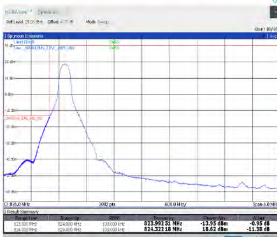
1-N26-824-849--15-5-L-4-CP-QPSK-Edge_1RB_Left-1@0-Ant1-seegraph-PASS-see graph
