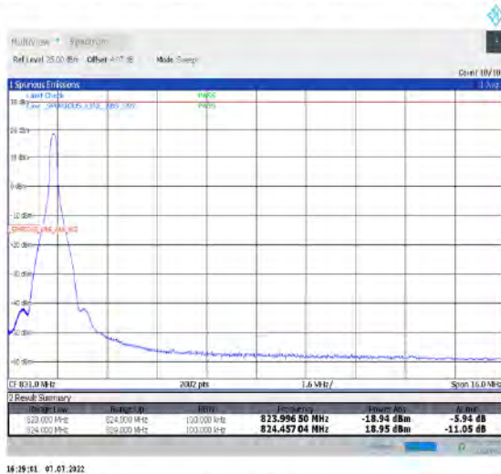
1-N26-824-849--15-15-L-4-CP-QPSK-Edge_1RB_Left-1@0-Ant1-seegraph-PASS-see graph
