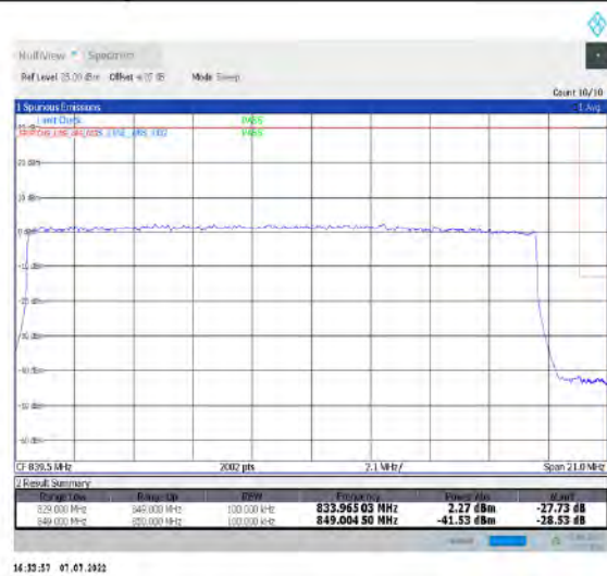
1-N26-824-849--15-20-H-3-DFT-PI2BPSK-Outer_Full-100@0-Ant1-seegraph-PASS-see graph
