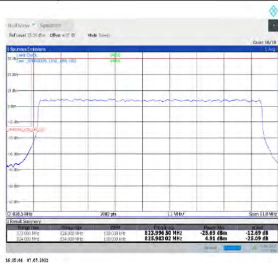
1-N26-824-849--15-10-L-3-DFT-PI2BPSK-Outer_Full-50@0-Ant1-seegraph-PASS-see graph
