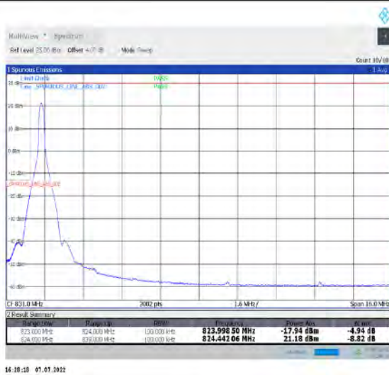
1-N26-824-849--15-15-L-1-DFT-PI2BPSK-Edge_1RB_Left-1@0-Ant1-seegraph-PASS-see graph
