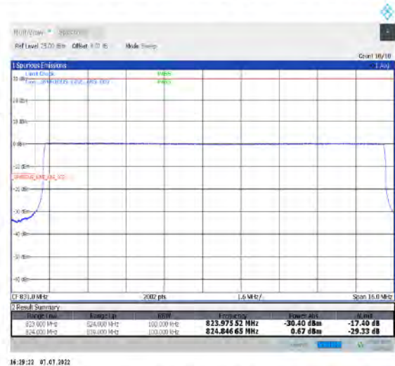
1-N26-824-849--15-15-L-6-CP-QPSK-Outer_Full-79@0-Ant1-seegraph-PASS-see graph
