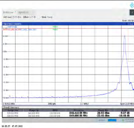
1-N26-824-849--15-20-H-2-DFT-PI2BPSK-Edge_1RB_Right-1@105-Ant1-seegraph-PASS-see graph
