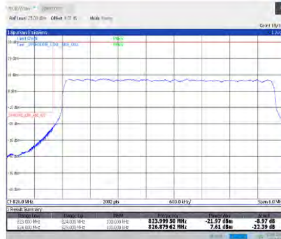
1-N26-824-849--15-5-L-3-DFT-PI2BPSK-Outer_Full-25@0-Ant1-seegraph-PASS-see graph
