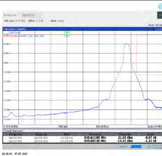
1-N26-824-849--15-5-H-2-DFT-PI2BPSK-Edge_1RB_Right-1@24-Ant1-seegraph-PASS-see graph
