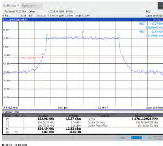
1-N26-824-849--15-5-L-1-DFT-QPSK-Outer_Full- 25@0-Ant1-4.482-5.000≤5-PASS
