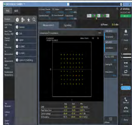
1-N26-824-849--15-20-M-8-CP-64QAM-Outer_Full-106@0-Ant1-see graph-PASS
