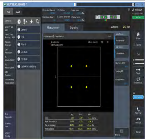
1-N26-824-849--15-20-M-6-CP-QPSK-Outer_Full-106@0-Ant1-see graph-PASS
