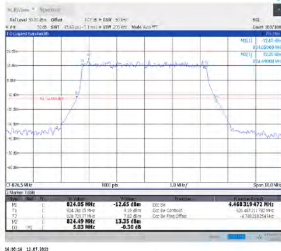
1-N26-824-849--15-5-L-2-DFT-PI2BPSK-Outer_Full- 25@0-Ant1-4.465-5.010-≤5-PASS
