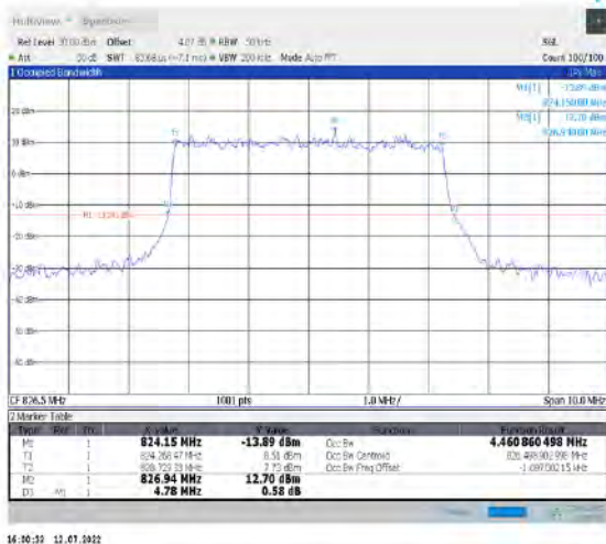
1-N26-824-849--15-5-L-3-DFT-16QAM-Outer_Full- 25@0-Ant1-4.469-4.860-≤5-PASS
