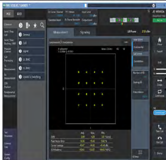
1-N26-824-849--15-20-M-7-CP-16QAM-Outer_Full-106@0-Ant1-see graph-PASS
