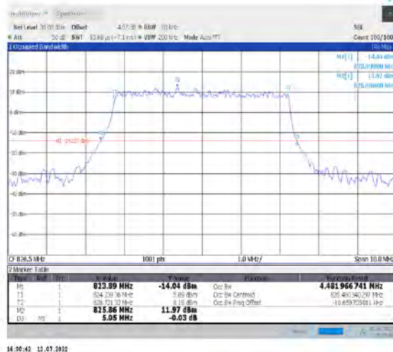
1-N26-824-849--15-5-L-4-DFT-64QAM-Outer_Full- 25@0-Ant1-4.471-5.070-≤5-PASS
