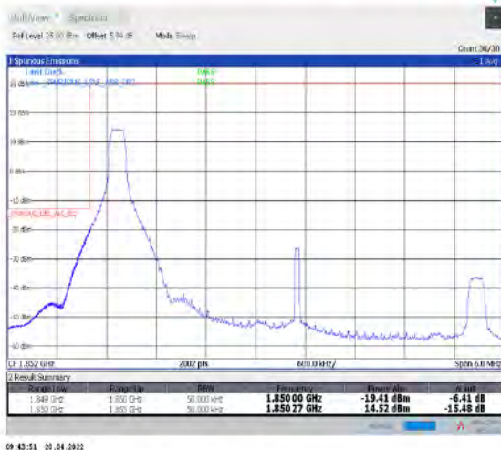
1-N25--15-5-L-4-CP-QPSK-Edge_1RB_Left-1@0-Ant1-seegraph-PASS-see graph
