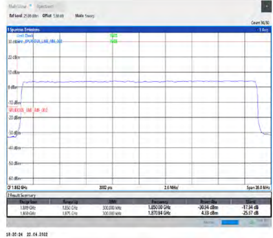
1-N25--15-25-L-3-DFT-PI2BPSK-Outer_Full-128@0-Ant1-seegraph-PASS-see graph
