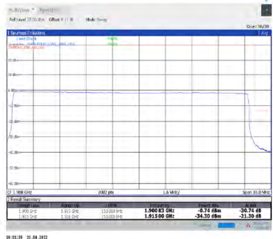
1-N25-15-15-H-6-CP-QPSK-Outer_Full-79@0-Ant1-seegraph-PASS-see graph
