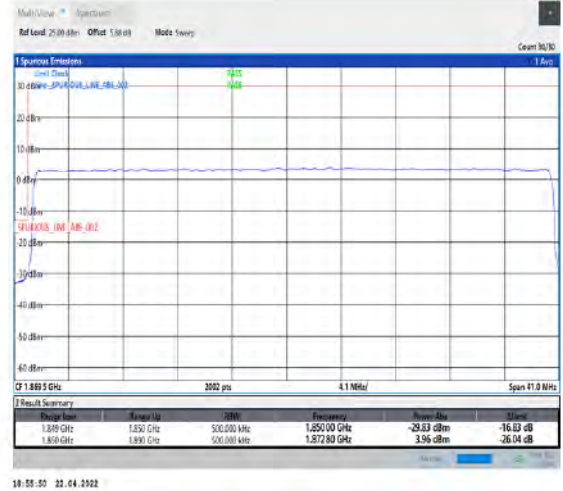
1-N25-15-40-L-3-DFT-PI2BPSK-Outer_Full-216@0-Ant1-seegraph-PASS-see graph
