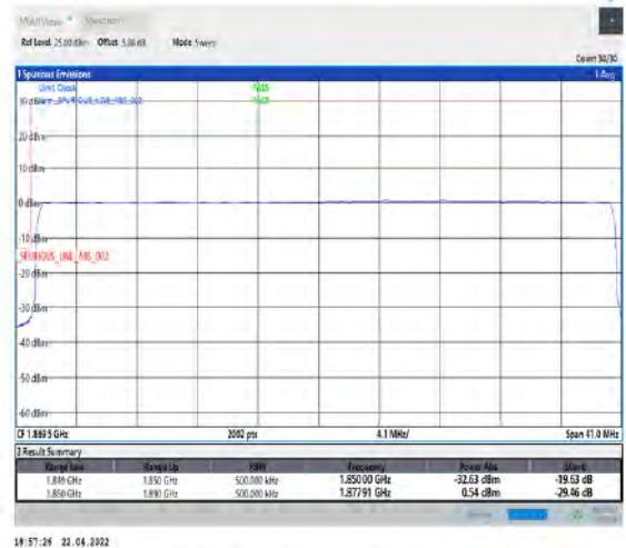
1-N25-15-40-L-6-CP-QPSK-Outer_Full-216@0-Ant1-seegraph-PASS-see graph
