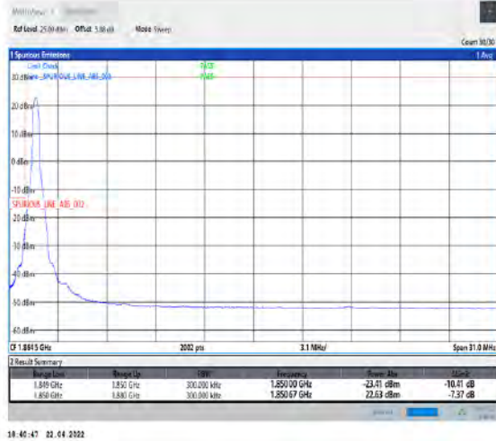
1-N25--15-30-L-1-DFT-PI2BPSK-Edge_1RB_Left-1@0-Ant1-seegraph-PASS-see graph
