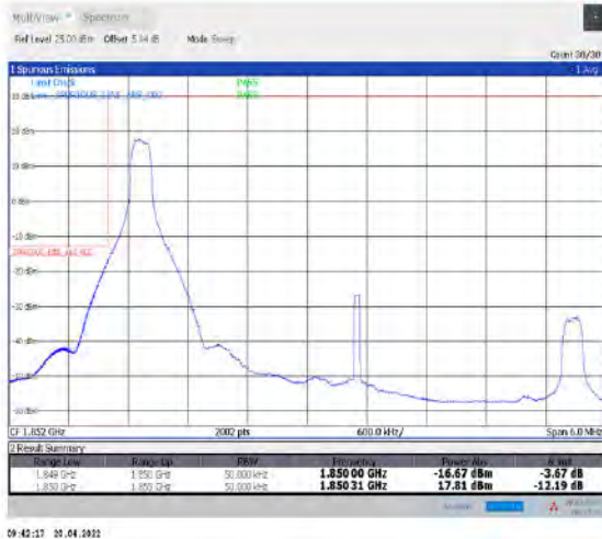
1-N25--15-5-L-1-DFT-PI2BPSK-Edge_1RB_Left-1@0-Ant1-seegraph-PASS-see graph
