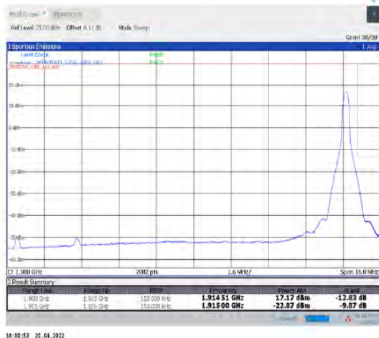
1-N25-15-15-H-5-CP-QPSK-Edge_1RB_Right-1@78-Ant1-seegraph-PASS-see graph
