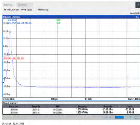
1-N25--15-30-L-4-CP-QPSK-Edge_1RB_Left-1@0-Ant1-seegraph-PASS-see graph
