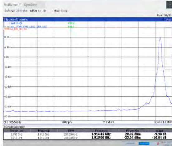
1-N25-15-20-H-2-DFT-PI2BPSK-Edge_1RB_Right-1@105-Ant1-seegraph-PASS-see graph
