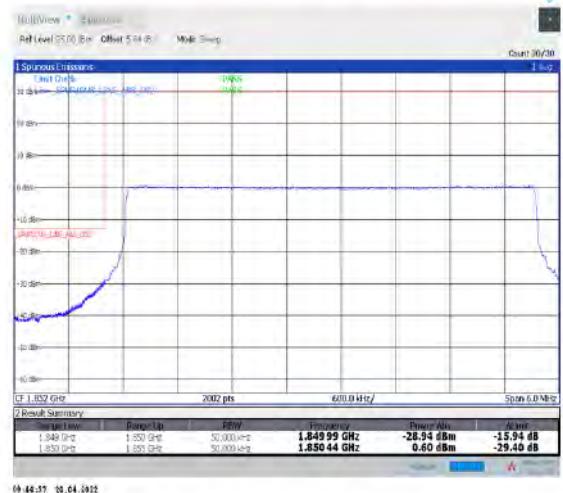
1-N25--15-5-L-6-CP-QPSK-Outer_Full-25@0-Ant1-seegraph-PASS-see graph
