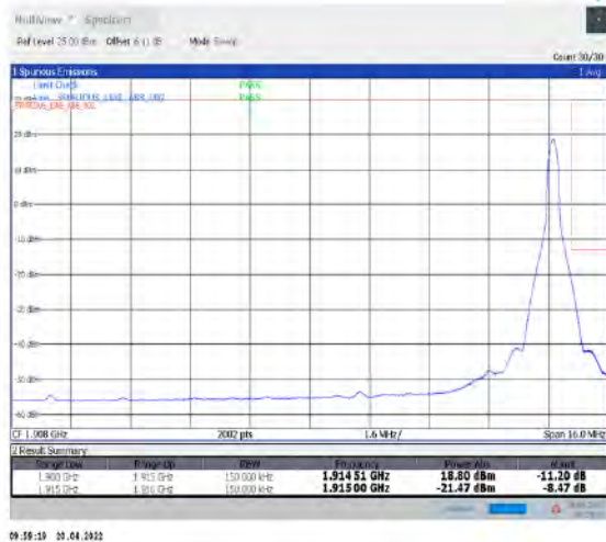
1-N25-15-15-H-2-DFT-PI2BPSK-Edge_1RB_Right-1@78-Ant1-seegraph-PASS-see graph
