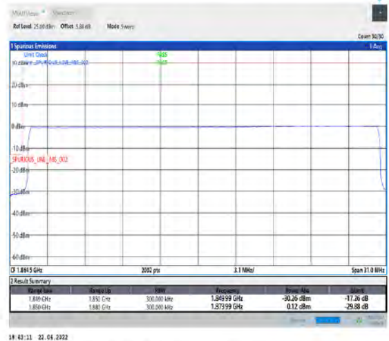
1-N25--15-30-L-6-CP-QPSK-Outer_Full-160@0-Ant1-seegraph-PASS-see graph
