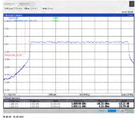
1-N25--15-5-L-3-DFT-PI2BPSK-Outer_Full-25@0-Ant1-seegraph-PASS-see graph
