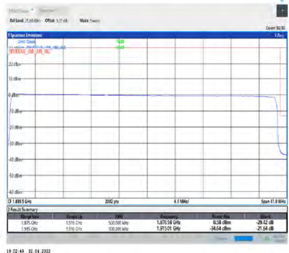
1-N25-15-40-H-6-CP-QPSK-Outer_Full-216@0-Ant1-seegraph-PASS-see graph
