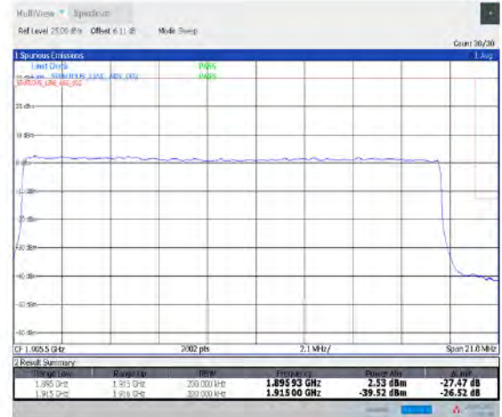
1-N25-15-20-H-3-DFT-PI2BPSK-Outer_Full-100@0-Ant1-seegraph-PASS-see graph
