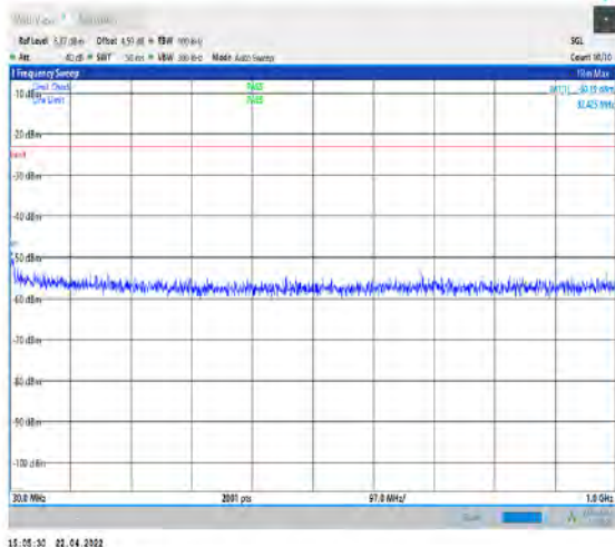
1-N25--15-40-L-1-DFT-PI2BPSK-Inner_1RB_Left- 1@1-30-1000-Ant1--50.19--23-PASS
