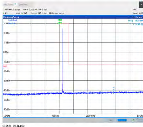
1-N25--15-40-L-1-DFT-PI2BPSK-Inner_1RB_Left- 1@1-1000-3000-Ant1--40.56--13-PASS
