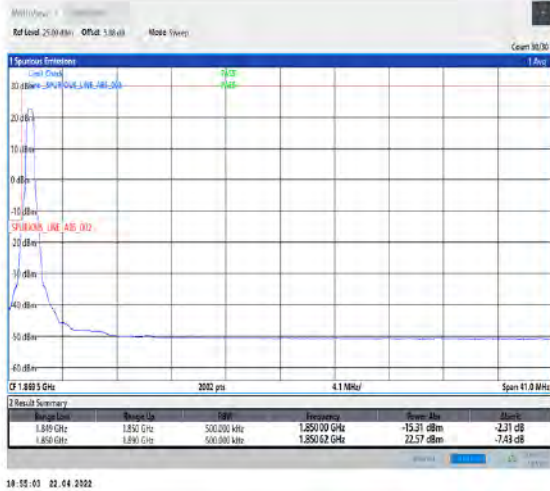
1-N25-15-40-L-1-DFT-PI2BPSK-Edge_1RB_Left-1@0-Ant1-seegraph-PASS-see graph
