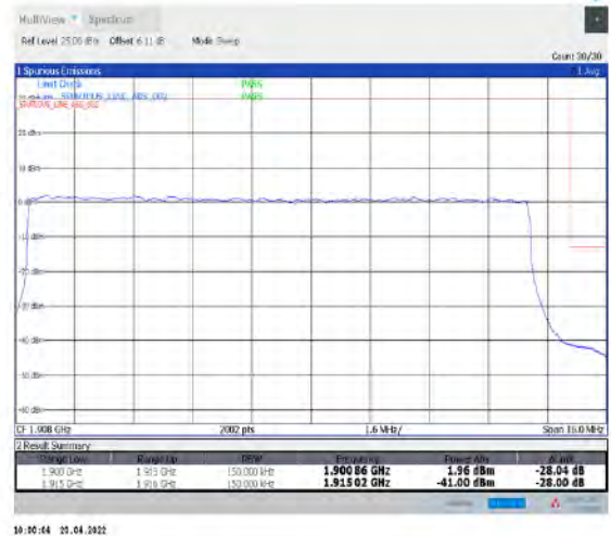
1-N25-15-15-H-3-DFT-PI2BPSK-Outer_Full-75@0-Ant1-seegraph-PASS-see graph
