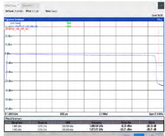
1-N25--15-30-H-6-CP-QPSK-Outer_Full-160@0-Ant1-seegraph-PASS-see graph
