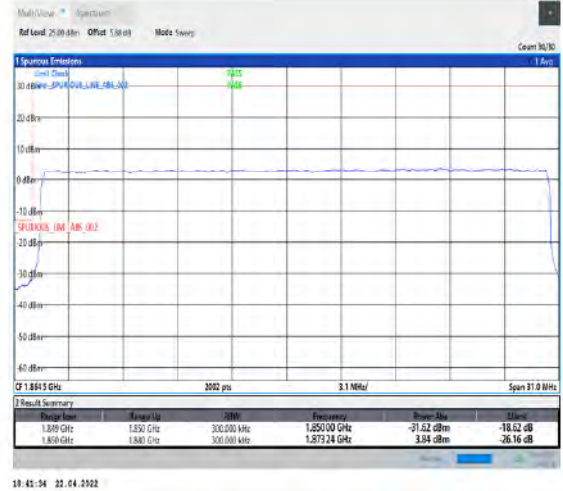
1-N25--15-30-L-3-DFT-PI2BPSK-Outer_Full-160@0-Ant1-seegraph-PASS-see graph
