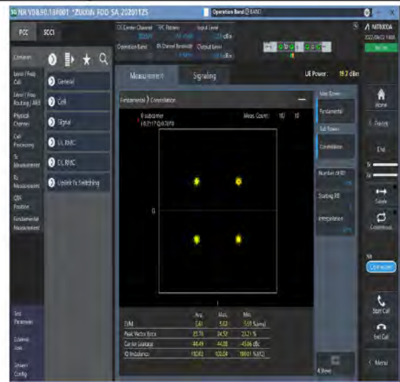
1-N25--15-40-M-6-CP-QPSK-Outer_Full-216@0-Ant1-see graph-PASS
