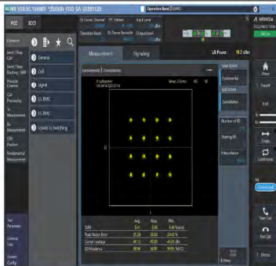
1-N25--15-40-M-7-CP-16QAM-Outer_Full-216@0-Ant1-see graph-PASS
