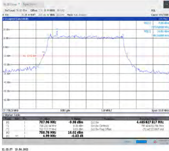
1-N14--15-5-L-1-DFT-QPSK-Outer_Full-25@0-Ant1-4.486-4.990-≤5-PASS
