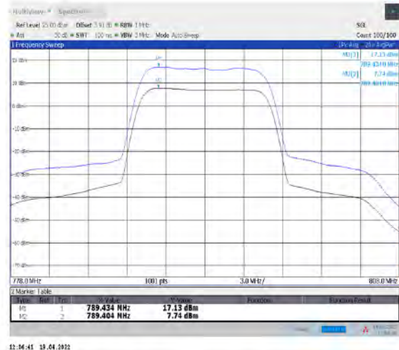
1-N14--15-10-M-2-CP-256QAM-Outer_Full-52@0-Ant1-9.39-100%-0.00-9.39-PASS-≤13
