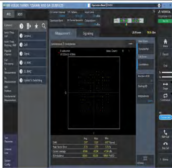
1-N14-PC3-15-10-M-5-DFT-256QAM-Outer_Full-50@0-Ant1-see graph-PASS
