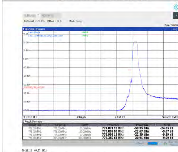
1-N13-PC3-15-10-L-4-CP-QPSK-Edge_1RB_Left- 1@0-Ant1-PASS-see graph
