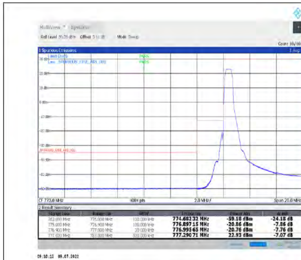
1-N13-PC3-15-10-L-1-DFT-PI2BPSK-Edge_1RB_Left- 1@0-Ant1-PASS-see graph
