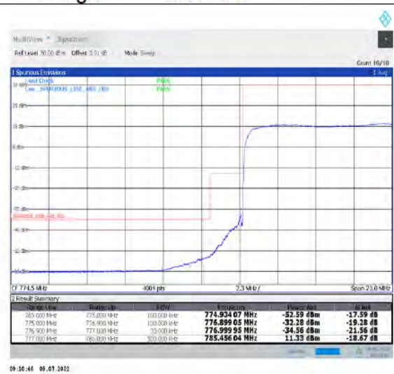
1-N13-PC3-15-10-L-3-DFT-PI2BPSK-Outer_Full- 50@0-Ant1-PASS-see graph
