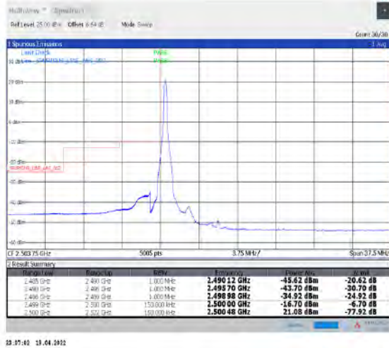
1-N7--15-15-L-1-DFT-PI2BPSK-Edge_1RB_Left-1@0-Ant1-PASS-see graph
