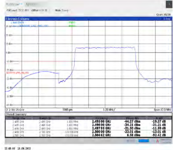
1-N7--15-5-L-3-DFT-PI2BPSK-Outer_Full-25@0-Ant1-PASS-see graph
