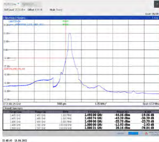
1-N7--15-5-L-1-DFT-PI2BPSK-Edge_1RB_Left-1@0-Ant1-PASS-see graph
