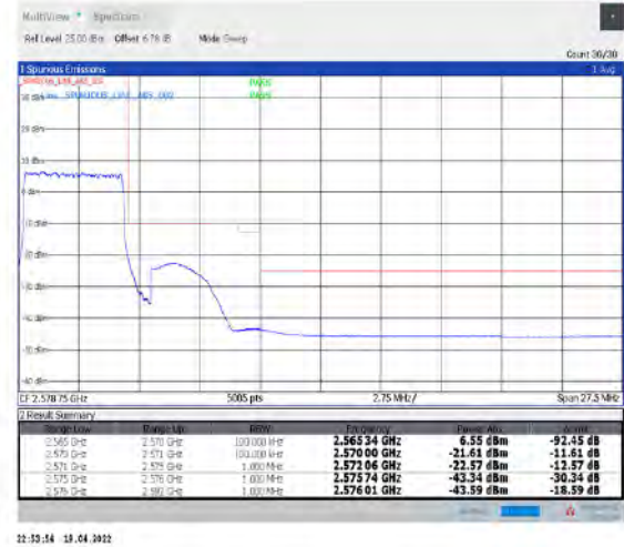
1-N7--15-5-H-3-DFT-PI2BPSK-Outer_Full-25@0-Ant1-PASS-see graph
