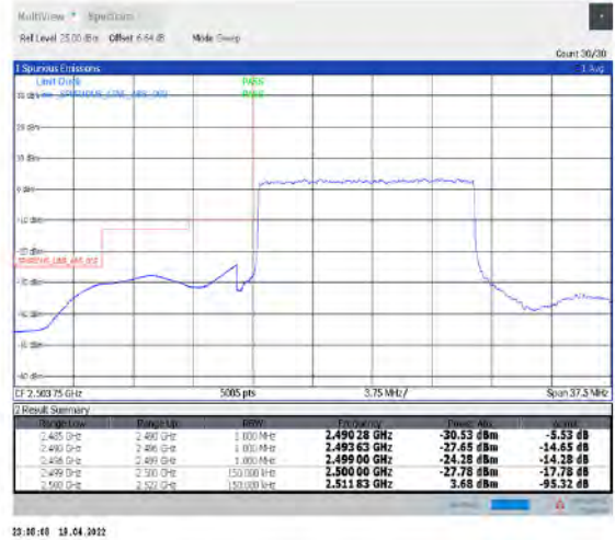
1-N7--15-15-L-3-DFT-PI2BPSK-Outer_Full-75@0-Ant1-PASS-see graph
