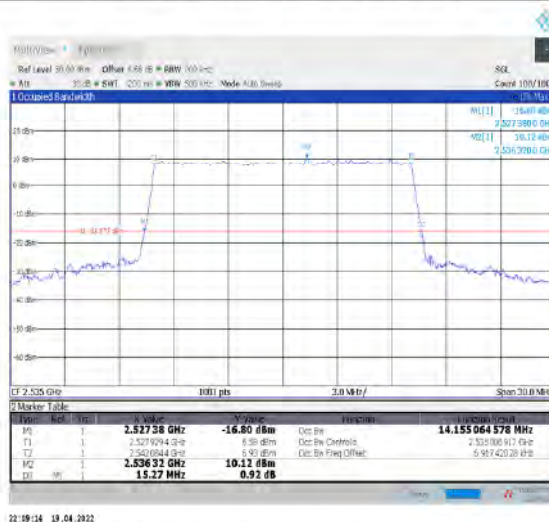
1-N7--15-15-M-9-CP-256QAM-Outer_Full-79@0- Ant1-14.155-15.270≤15-PASS
