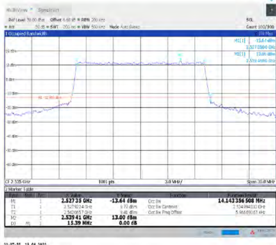
1-N7--15-15-M-6-CP-QPSK-Outer_Full-79@0-Ant1- 14.143-15.390-<15-PASS
