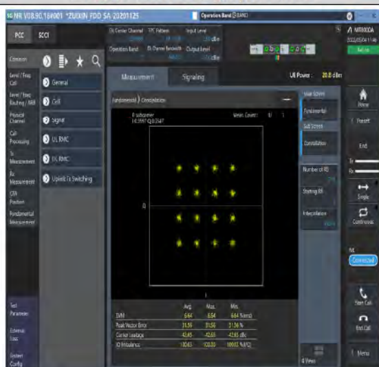
1-N7-PC3-15-40-M-7-CP-16QAM-Outer_Full-216@0- Ant1-see graph-PASS
