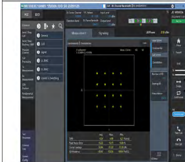
1-N5--15-20-M-7-CP-16QAM-Outer_Full-106@0-Ant1-see graph-PASS
