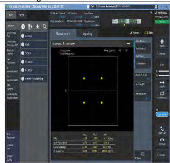
1-N5--15-20-M-6-CP-QPSK-Outer_Full-106@0-Ant1-see graph-PASS
