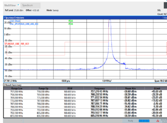
Band14-5MHz-QPSK-23305-25RB#0
