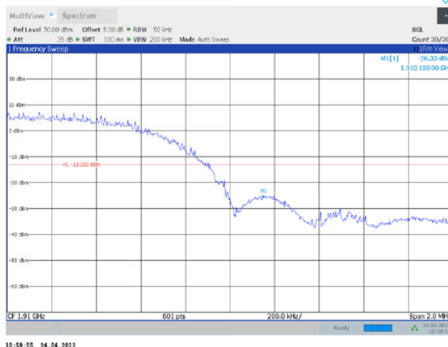
Band2-9538
