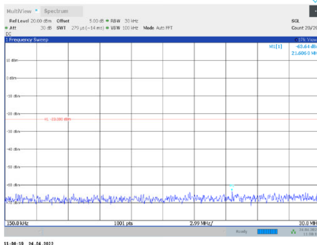
Band2-9262-0.15~30MHz
