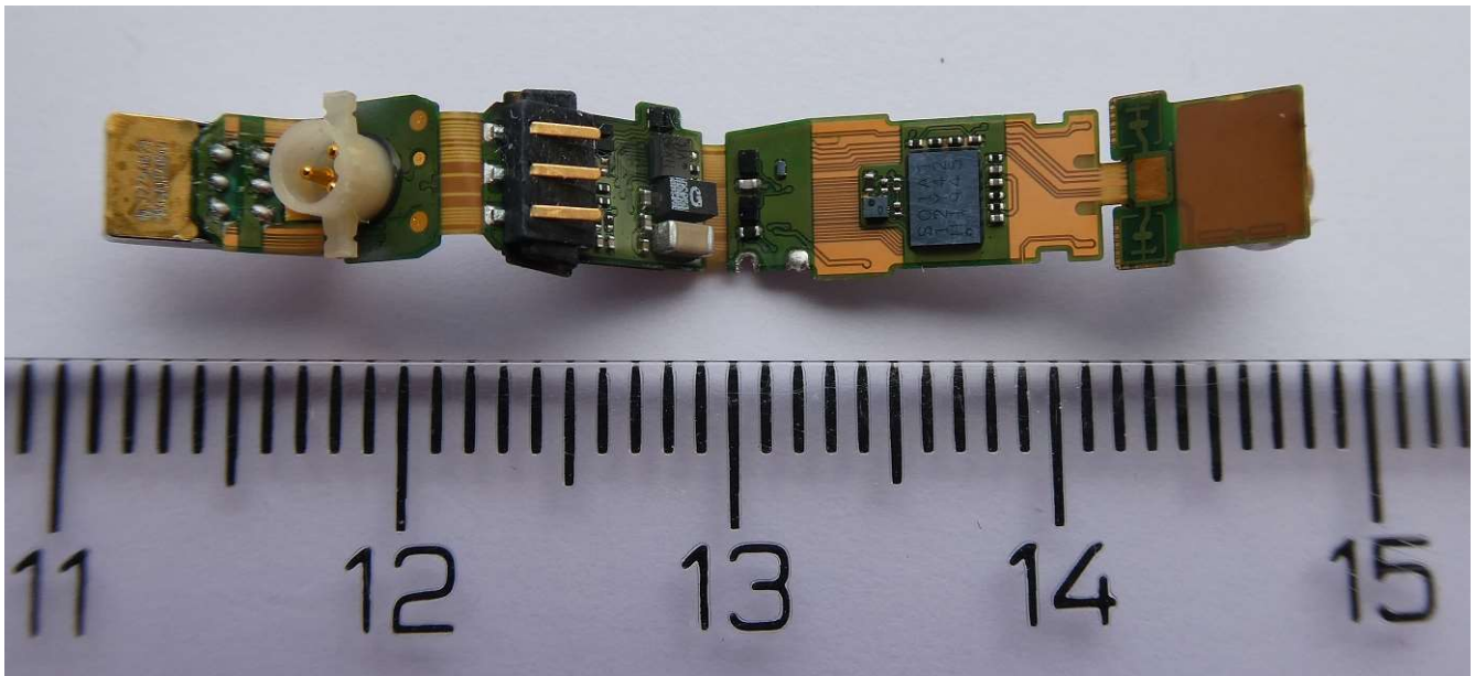
PCB showing the connector side
