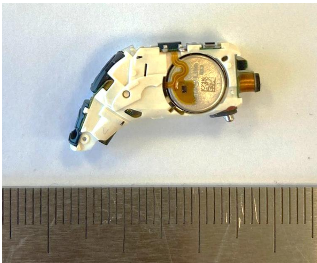
Picture 2 The hearing instrument module stack up – left side.
