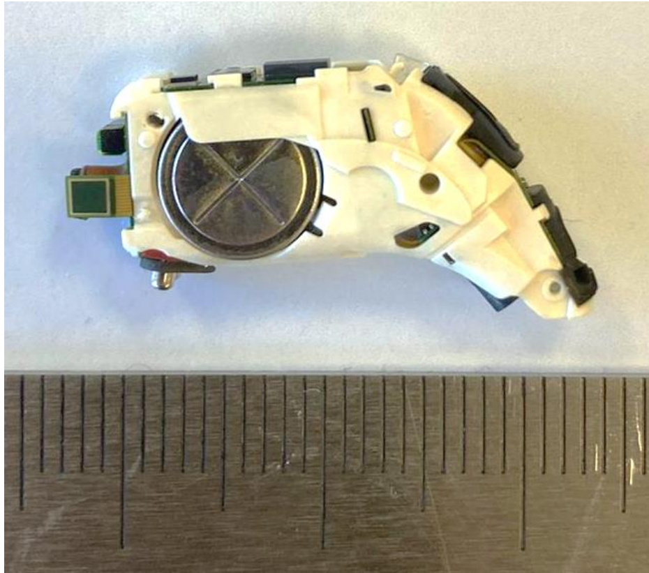
Picture 3 The hearing instrument module stack up – right side.
