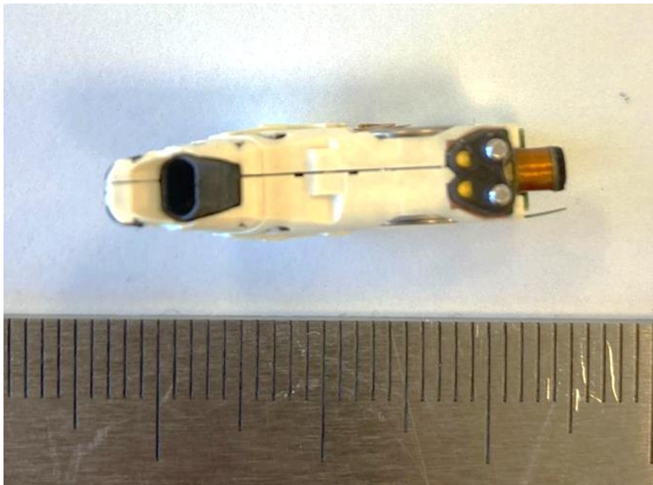
Picture 4 The hearing instrument module stack up – bottom side with interface for speakers (left). Telecoil at right.
