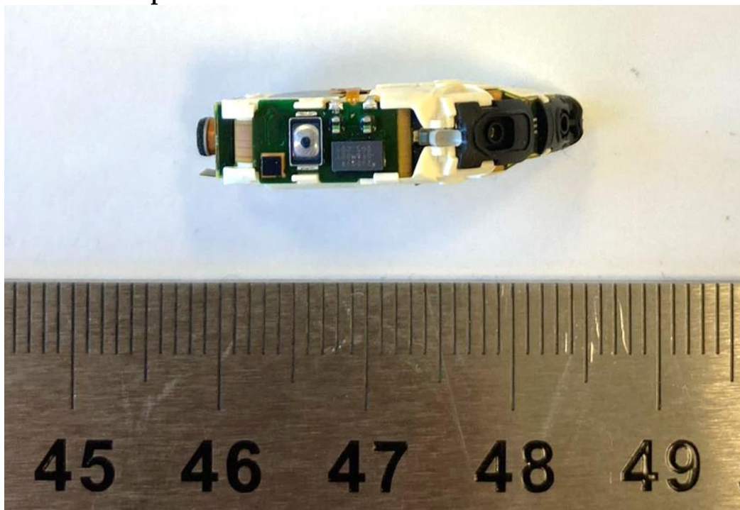
Picture 1 The hearing instrument module stack up – top side.
