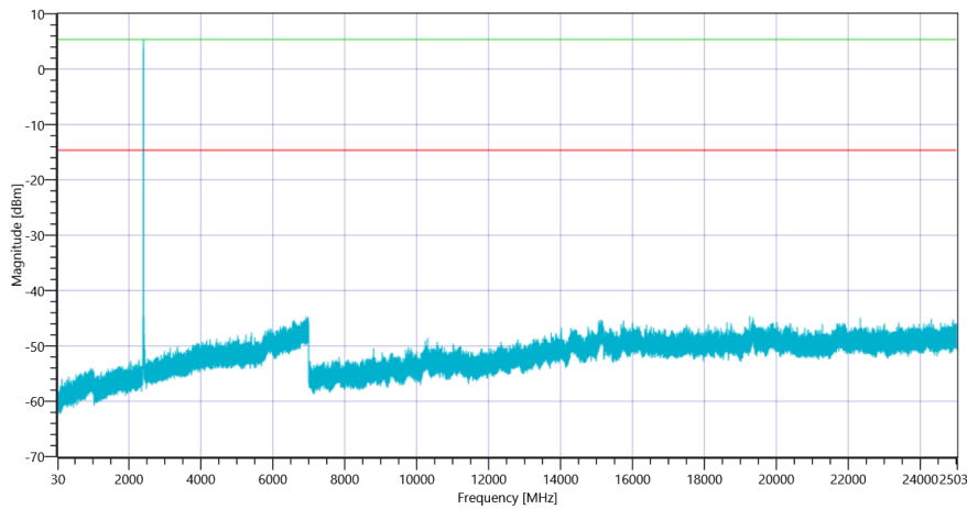
Plot_FCC Part 15.247 TX Spurious Conducted ~ BT LE 2 Msps 2404_20092021_141413.png
