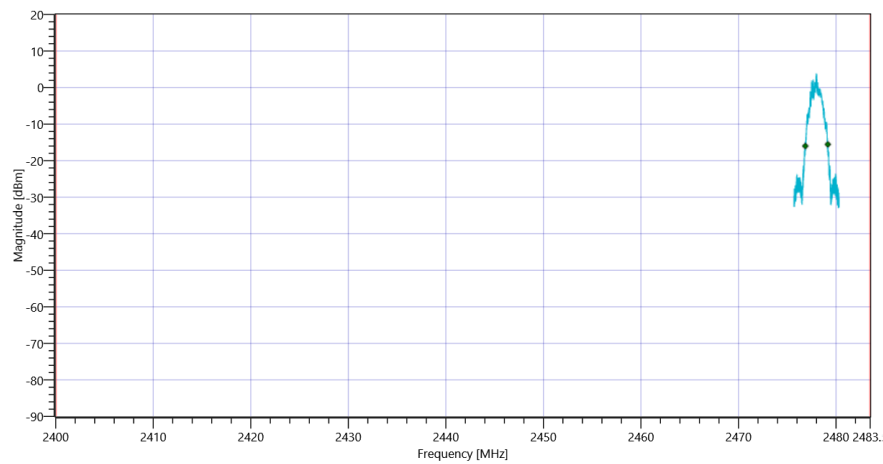
Plot_FCC Part 15.247 Bandwidth 99PCT-20dB ~ BT LE 2 Msps 20dB_20092021_151347.png
