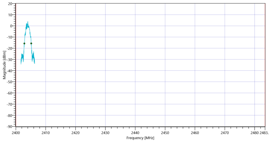
Plot_FCC Part 15.247 Bandwidth 99PCT-20dB ~ BT LE 2 Msps_20092021_140829.png
