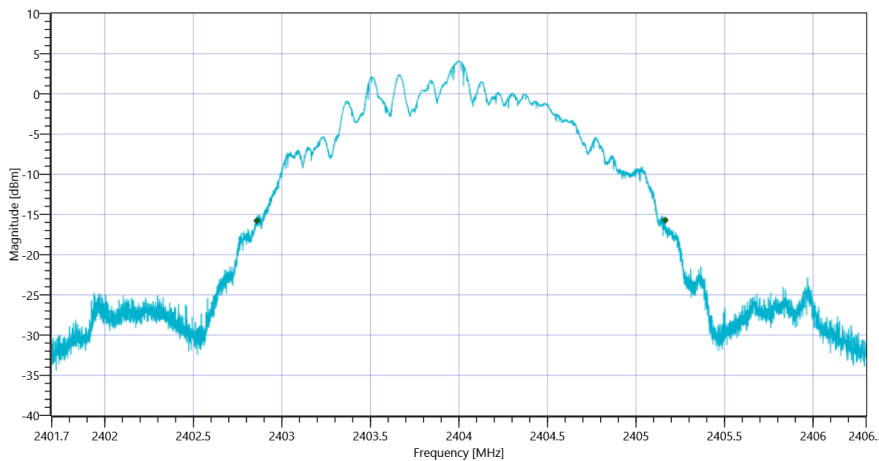
Plot_FCC Part 15.247 Bandwidth 99PCT-20dB ~ BT LE 2 Msps 20dB_20092021_140823.png
