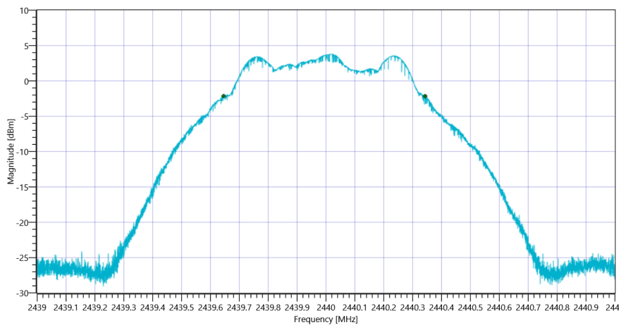
Plot_FCC Part 15.247 Maximum Peak Conducted Output Power DTS ~ BT LE 1 Msps DTS BW_20092021_130721.png
