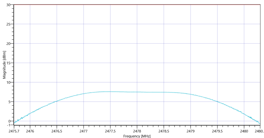
Plot_FCC Part 15.247 Maximum Peak Conducted Output Power DTS ~ BT LE 2 Msps_20092021_151113.png
