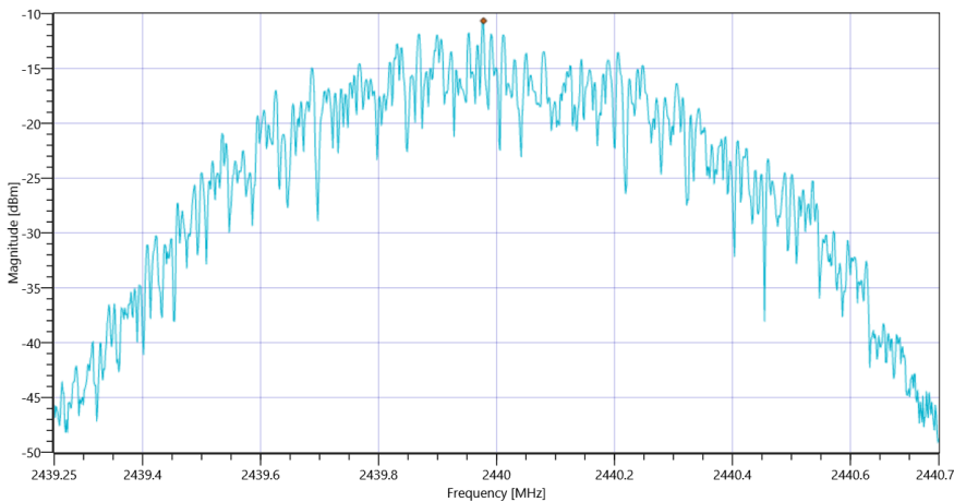
Plot_FCC Part 15.247 Peak Power Spectral Density DTS ~ BT LE 1 Msps_20092021_130906.png
