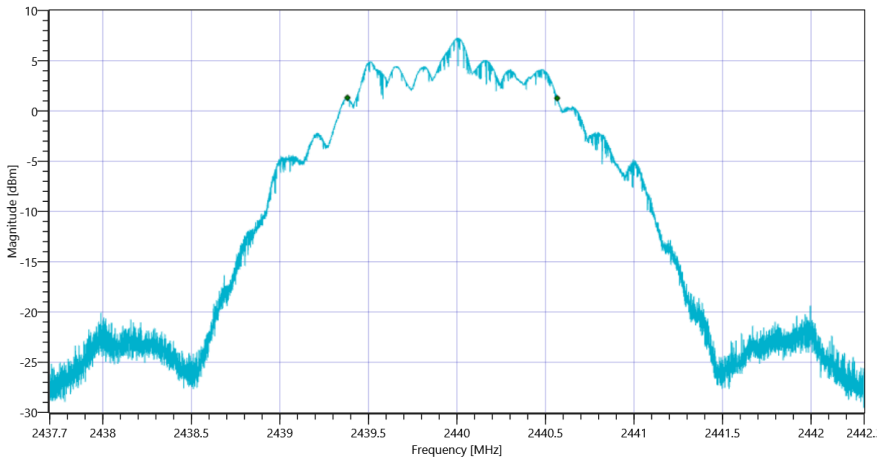
Plot_FCC Part 15.247 Bandwidth 6dB DTS ~ BT LE 2 Msps_20092021_144231.png
