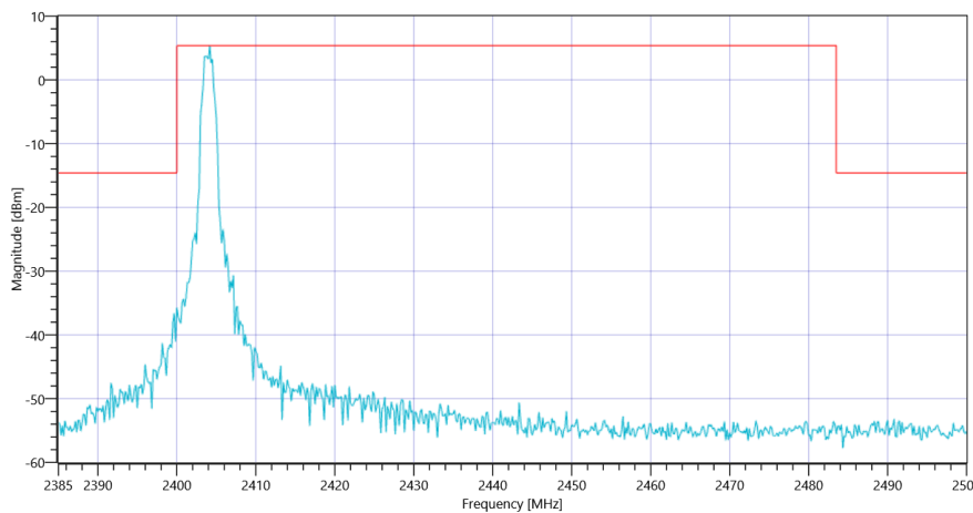
Plot_FCC Part 15.247 TX Spurious Conducted ~ BT LE 2 Msps 2404_20092021_141418.png
