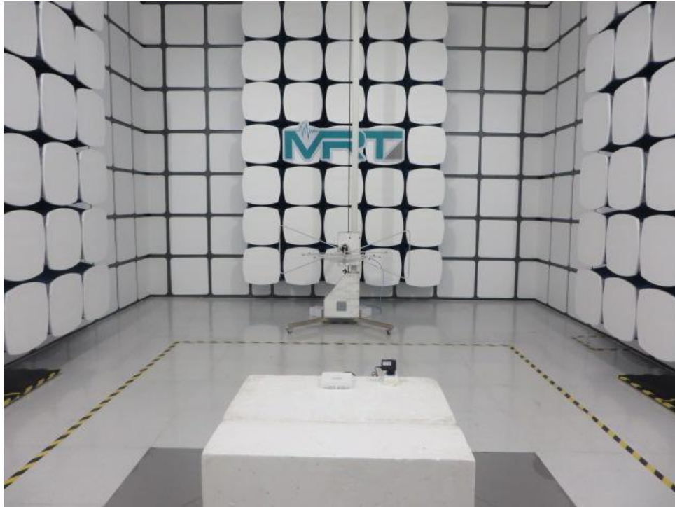
FCC 15B RE Above 1GHz
