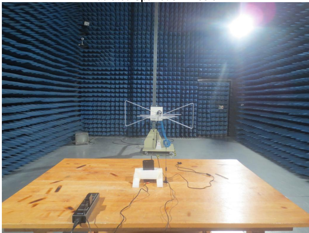
Model No.: TM5HLM Radiated Spurious Emission
