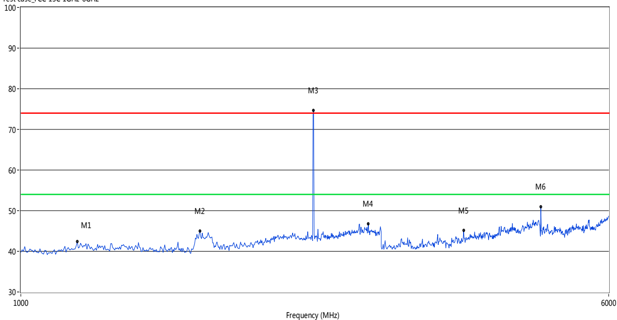
RE Test case_FCC 15C 1GHz-6GHz
