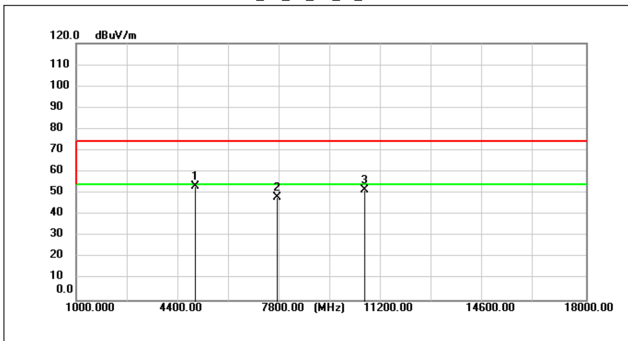
BLE_1M_TX_CH_39_Verical
