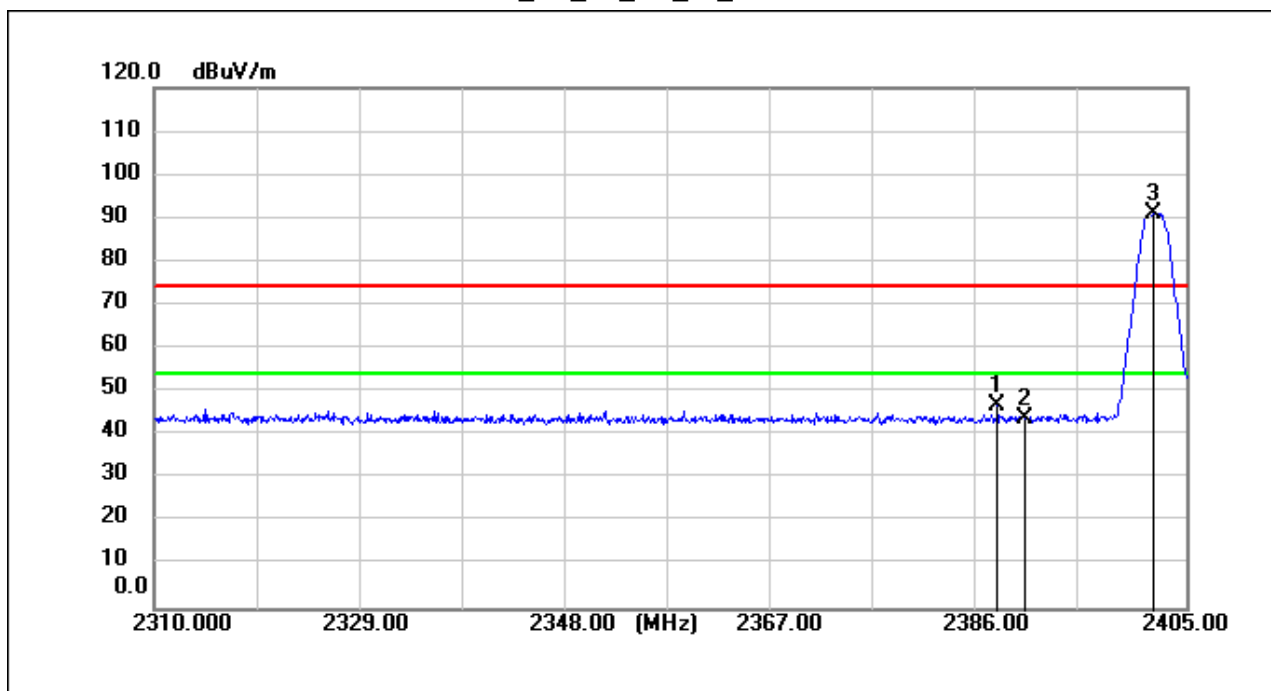
BLE_2M_TX_CH_00_Vertical
