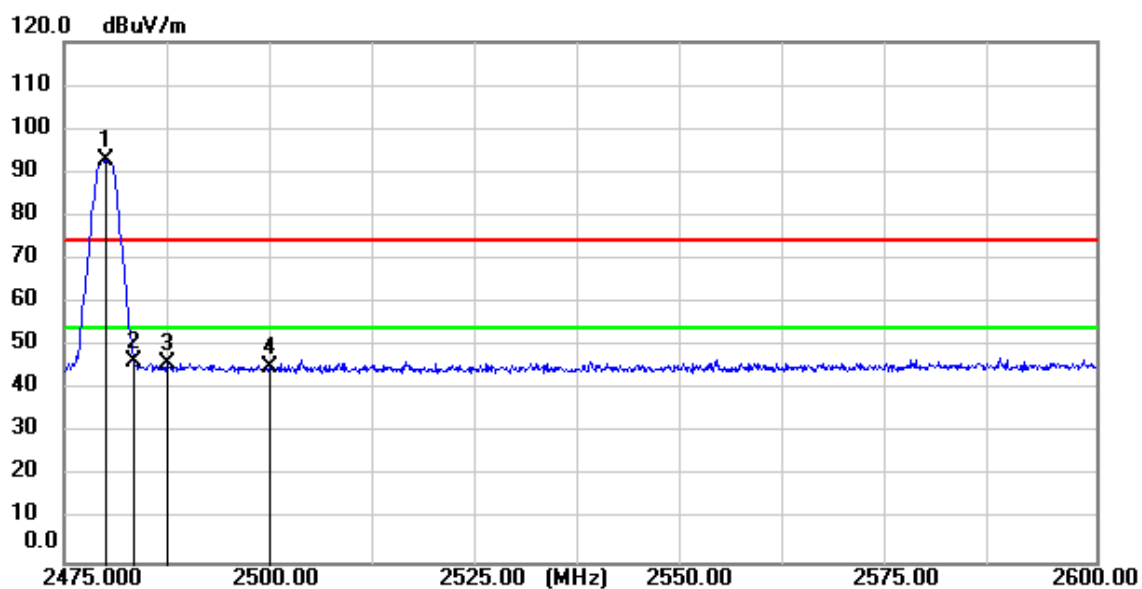
BLE_2M_TX_CH_39_Horizontal_Peak
