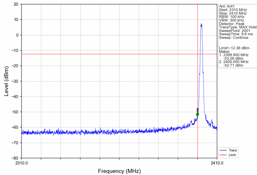
1M_LCH_2402MHz_Ant1_NTNV
