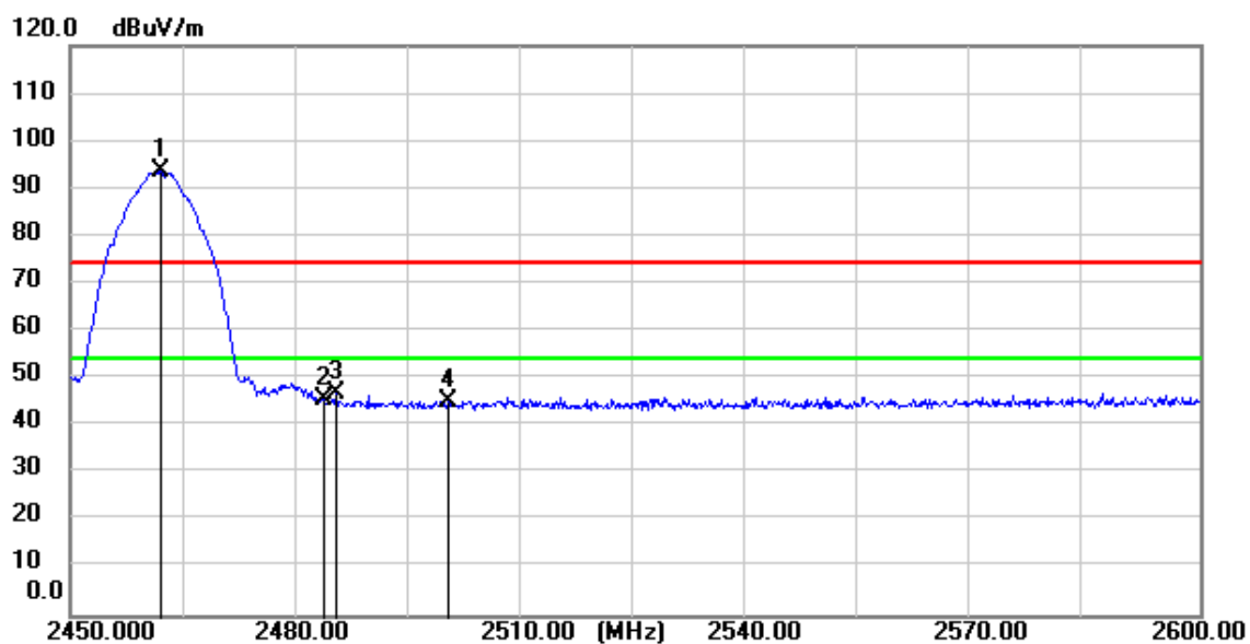
11b_TX_CH_11_Vertical_Peak
