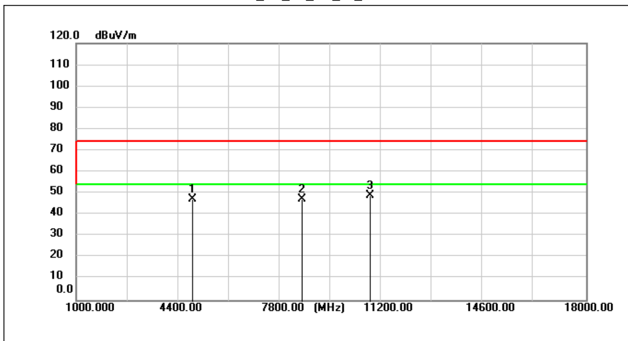
BLE_2M_TX_CH_19_Vertical
