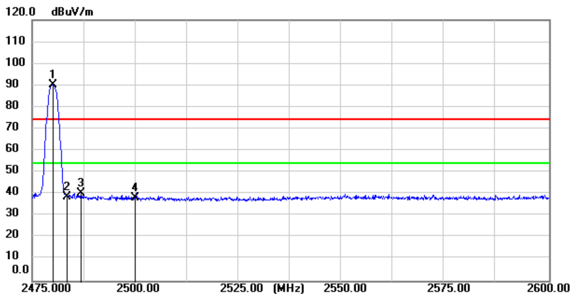
BLE_1M_TX_CH_39_Verical
