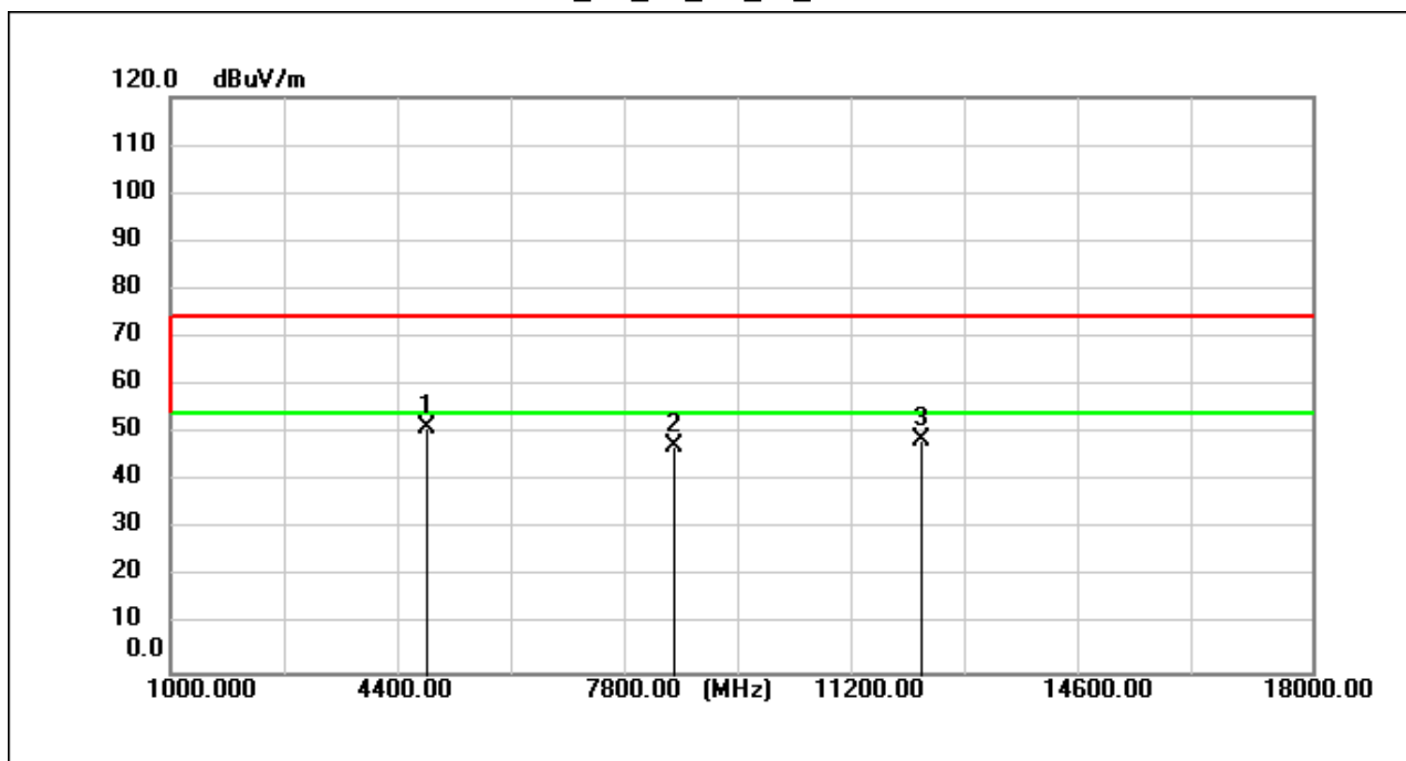
BLE_1M_TX_CH_00_Verical
