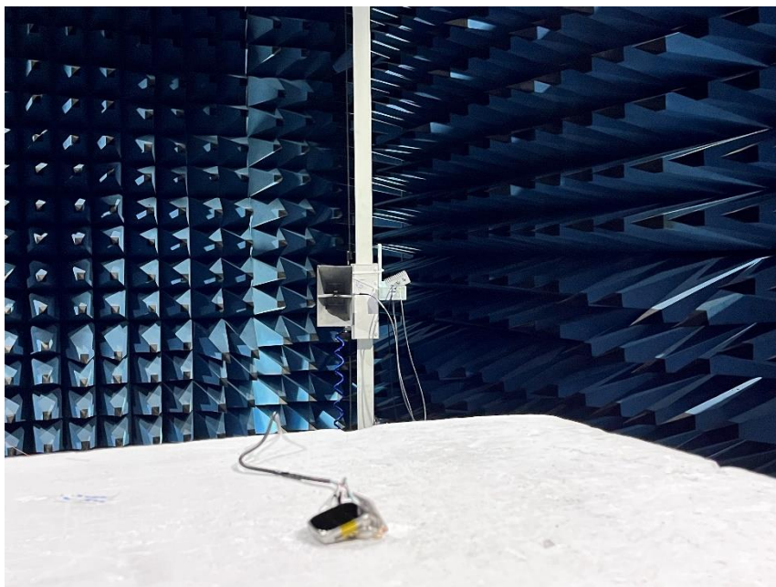
Radiated Test Setup Above 1GHz
