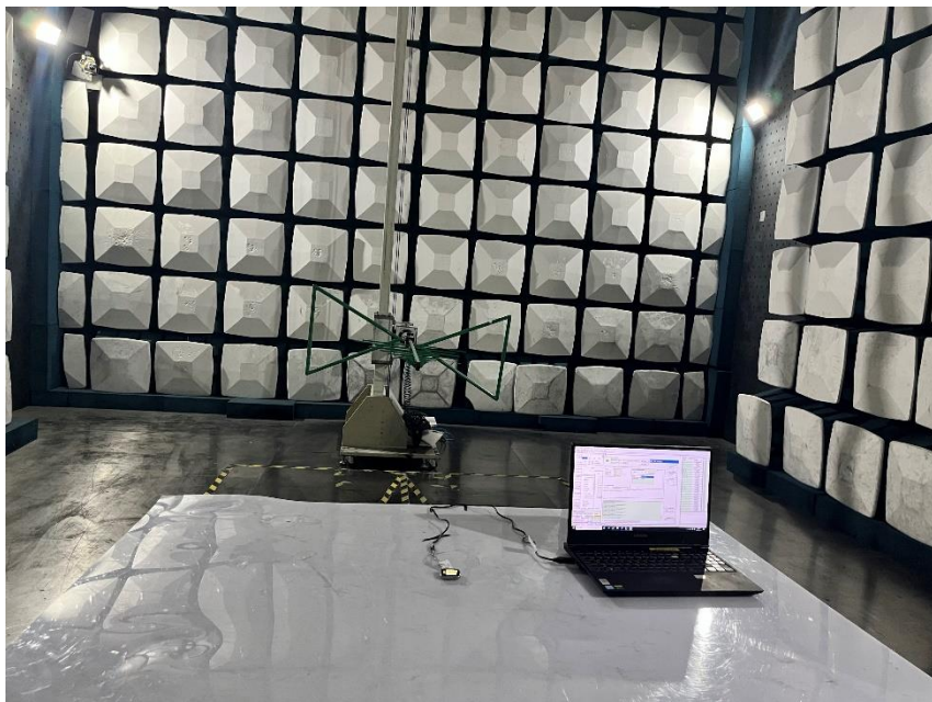
Radiated Test Setup Below 1GHz
