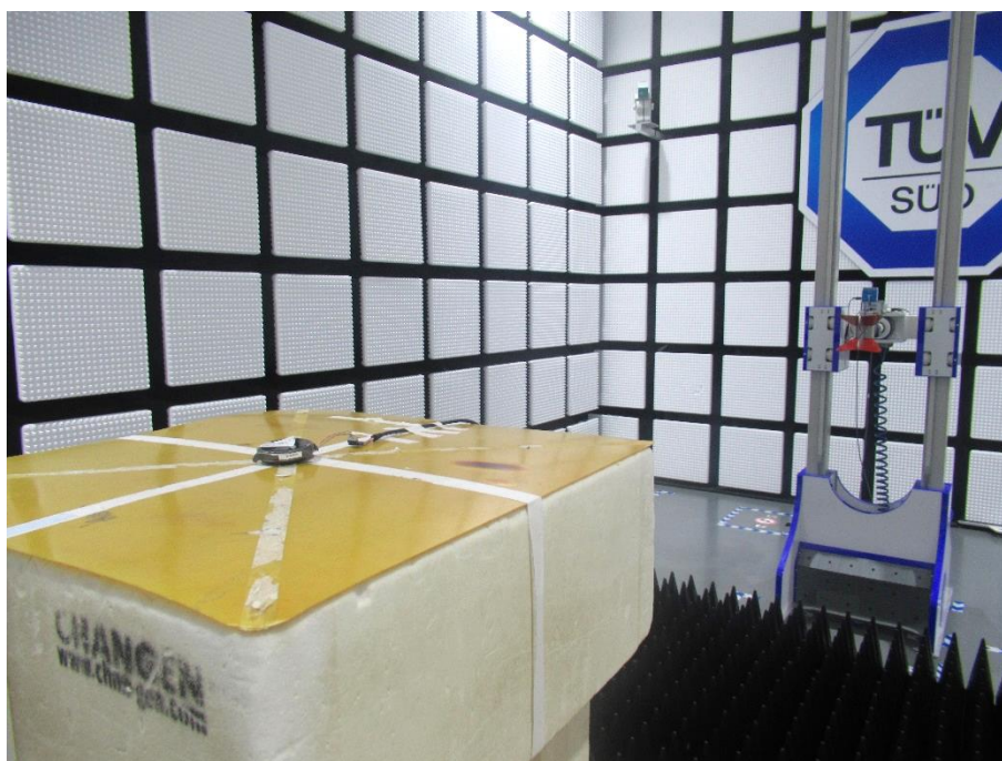
Above 1GHz RSE Setup
