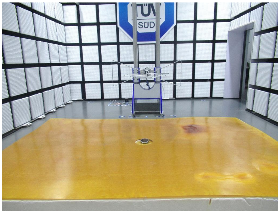
Below 1GHz RSE Setup
