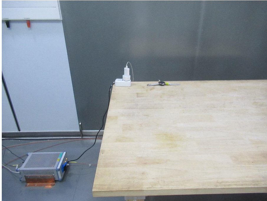
Conducted emission AC power port Setup
