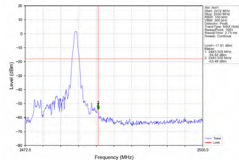
GFSK_DH5_HCH_2480MHz_Ant1_NTNV
