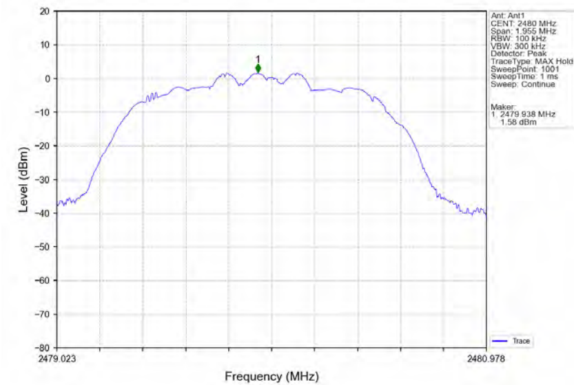
8DPSK_3DH5_HCH_2480MHz_Ant1_NTNV
