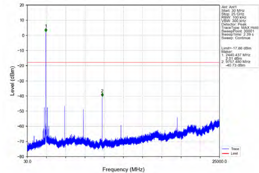
Pi/4DQPSK_2DH5_MCH_2441MHz_Ant1_NTNV
