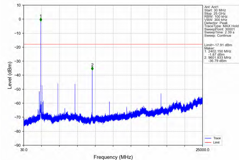
8DPSK_3DH5_LCH_2402MHz_Ant1_NTNV
