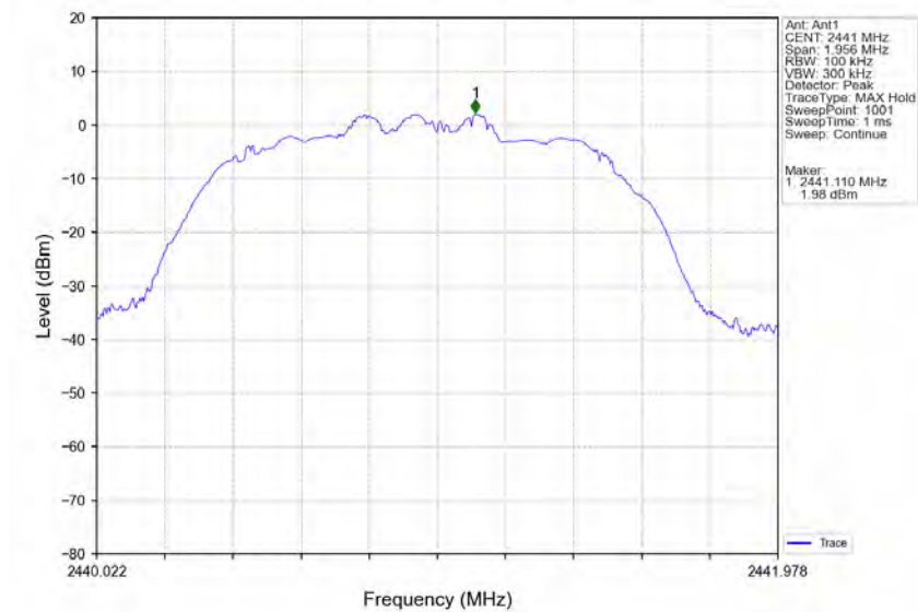
8DPSK_3DH5_MCH_2441MHz_Ant1_NTNV
