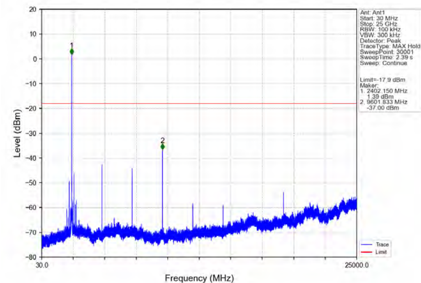
GFSK_DH5_LCH_2402MHz_Ant1_NTNV
