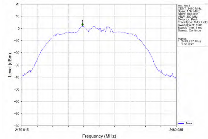
Pi/4DQPSK_2DH5_HCH_2480MHz_Ant1_NTNV
