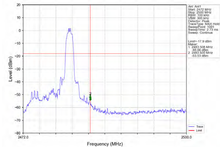
8DPSK_3DH5_HCH_2480MHz_Ant1_NTNV
