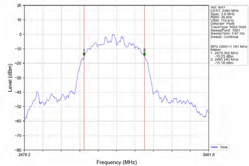
8DPSK_3DH5_HCH_2480MHz_Ant1_NTNV
