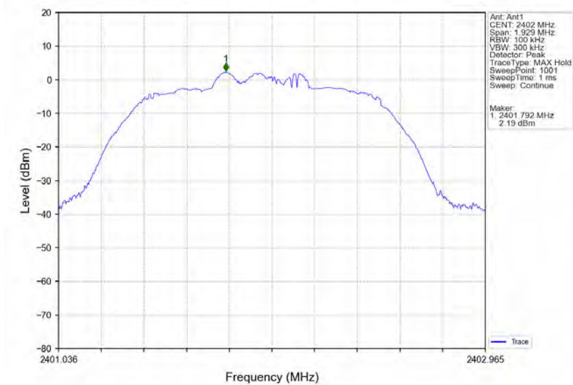
Pi/4DQPSK_2DH5_LCH_2402MHz_Ant1_NTNV
