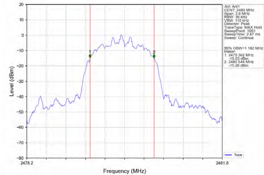
8DPSK_3DH5_HCH_2480MHz_Ant1_NTNV
