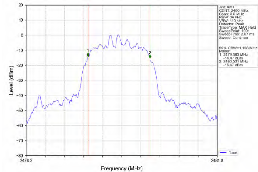
Pi/4DQPSK_2DH5_HCH_2480MHz_Ant1_NTNV
