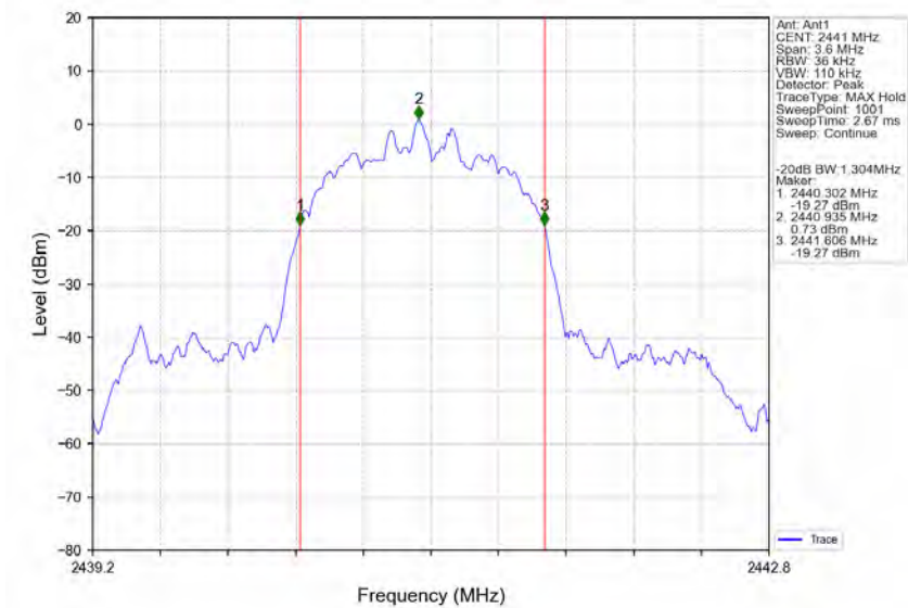
8DPSK_3DH5_MCH_2441MHz_Ant1_NTNV
