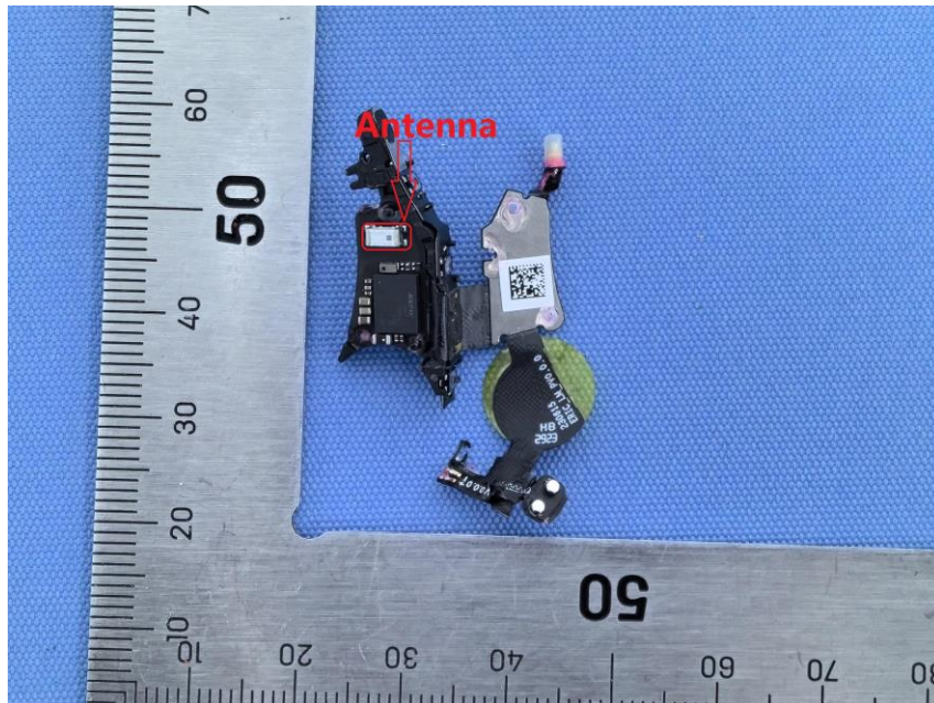
Left Earbud
