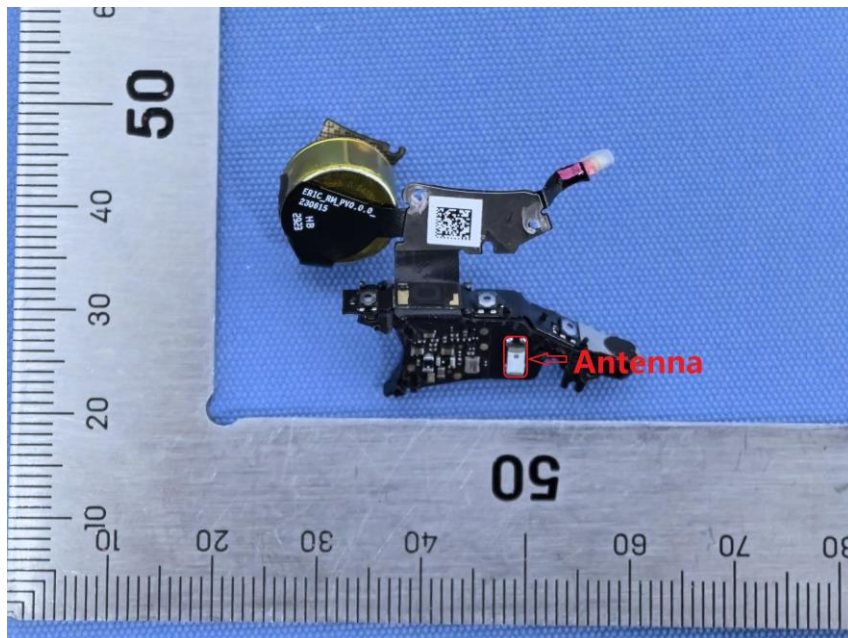
Right Earbud
