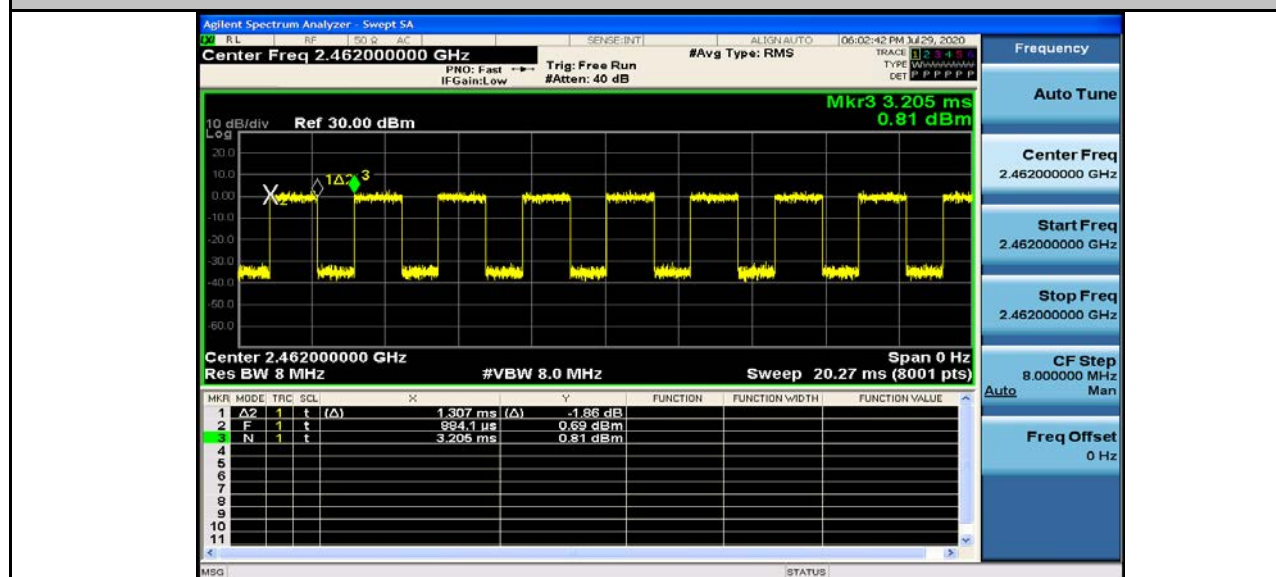
Duty Cycle_11N20SISO_2462_Ant1
