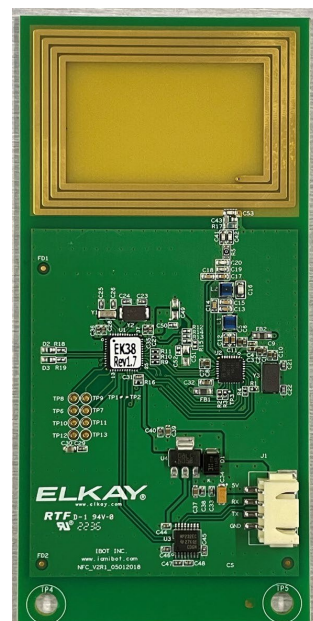
Filter NFC Board w/trace antenna
