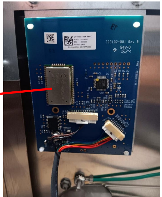
Endpoint (LoRa) Board w/trace antenna
