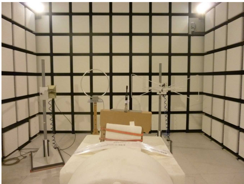
Photo 4: BTLE test setup in the anechoic chamber
