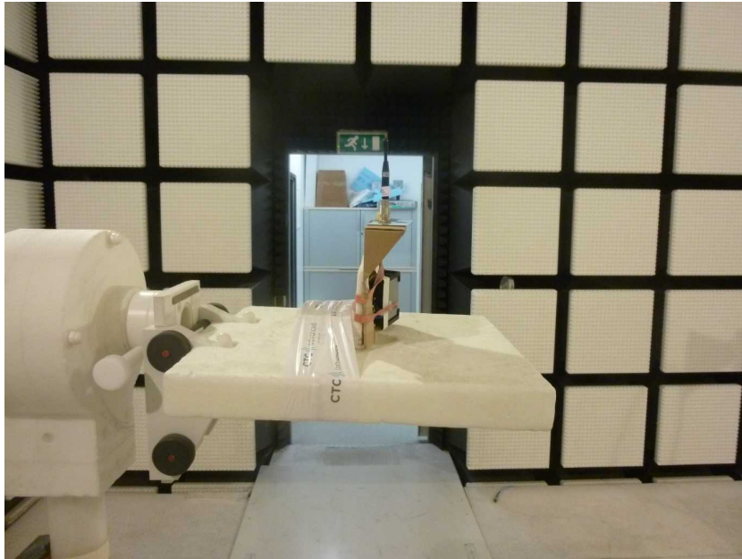
Photo 3: BTLE test setup in the anechoic chamber
