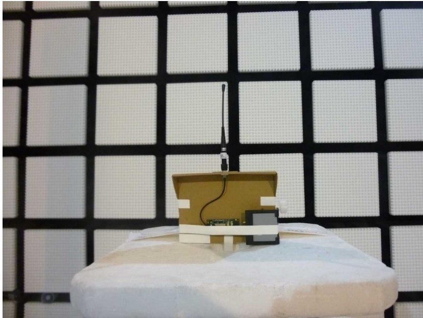
Photo 9: 902-928 MHz proprietary test setup at the anechoic chamber
