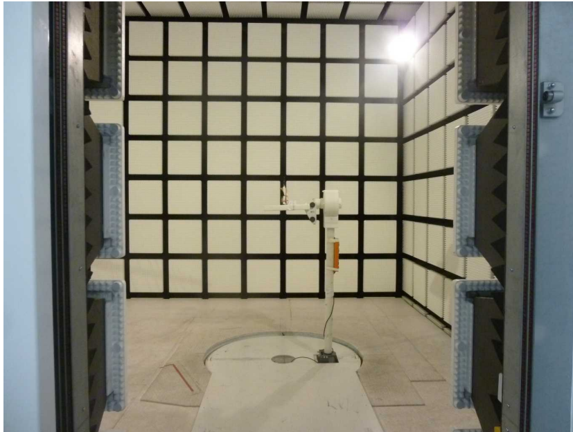
Photo 1: BTLE test setup in the anechoic chamber
