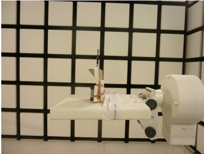
Photo 5: BTLE test setup in the anechoic chamber
