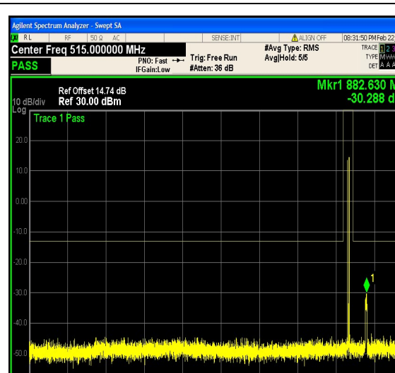
1-N5-PC3-15-5-M-23-CP-64QAM-Edge_1RB _Right-1@24-30-1000-Ant1--30.29--13-PASS
