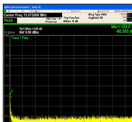
1-N5-PC3-15-5-M-19-CP-16QAM-Edge_1RB _Left-1@0-3000-12000-Ant1--42.38--13-PASS
