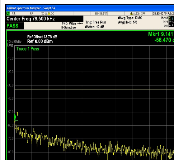
1-N5-PC3-15-5-M-22-CP-64QAM-Edge_1RB
