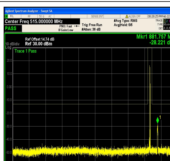
1-N5-PC3-15-5-M-19-CP-16QAM-Edge_1RB _Left-1@0-30-1000-Ant1--28.22--13-PASS
