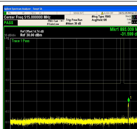
1-N5-PC3-15-5-H-8-DFT-16QAM-Edge_1RB _Right-1@24-30-1000-Ant1--31.60--13-PASS
