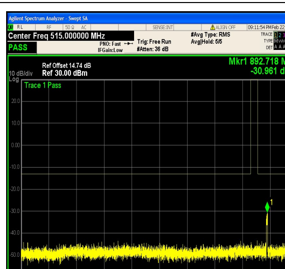
1-N5-PC3-15-5-H-18-CP-QPSK-Outer_Full-2 5@0-30-1000-Ant1--30.96--13-PASS
