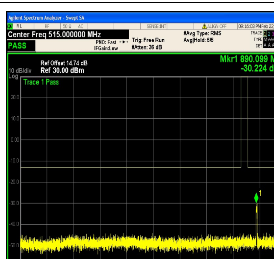
1-N5-PC3-15-5-H-20-CP-16QAM-Edge_1RB _Right-1@24-30-1000-Ant1--30.22--13-PASS
