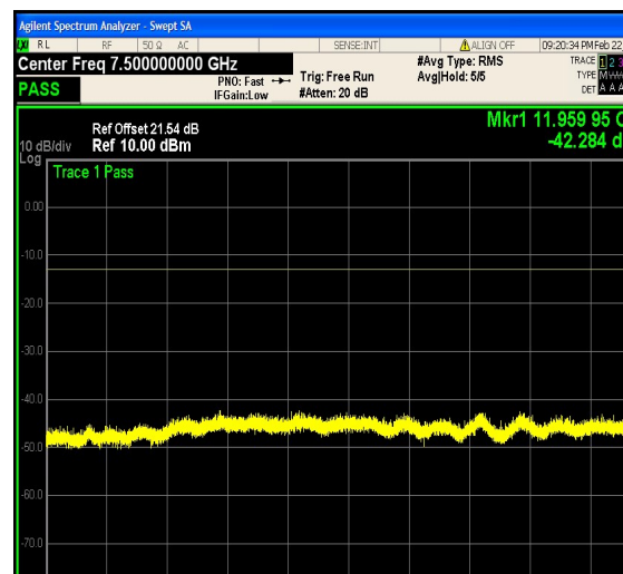
1-N5-PC3-15-5-H-22-CP-64QAM-Edge_1RB _Left-1@0-3000-12000-Ant1--42.28--13-PASS
