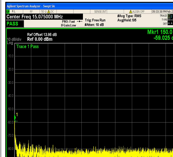
1-N5-PC3-15-10-L-3-DFT-PI2BPSK-Outer_F ull-50@0-0.15-30-Ant1--59.02--23-PASS
