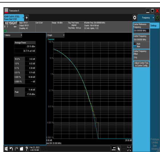
1-N5-PC3-15-20-L-5-DFT-256QAM-Outer_Fu ll-100@0-8.38-100%-0.00-8.38-PASS-≤13
