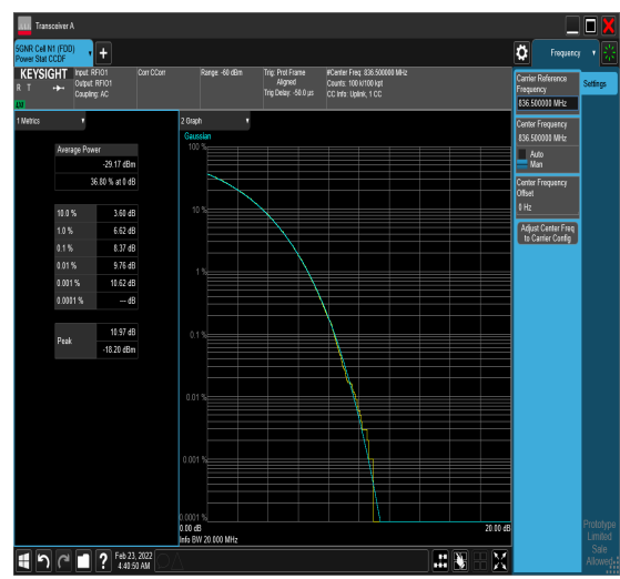
1-N5-PC3-15-15-M-9-CP-256QAM-Outter_Ful-I-79 79@0-8.37-100%-0.00-8.37-PASS-≤13
