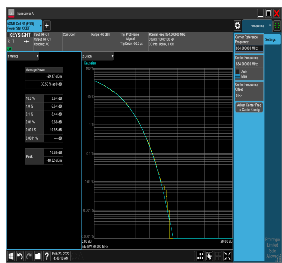
1-N5-PC3-15-20-L-9-CP-256QAM-Outer_Full
