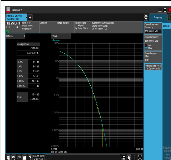
1-N5-PC3-15-20-L-2-DFT-QPSK-Outet_Full- 100@0-8.39-100%-0.00-8.39-PASS-≤13 1-N5-PC3-15-20-L-3-DFT-16QAM-Outet_Full -100@0-8.38-100%-0.00-8.38-PASS-≤13
