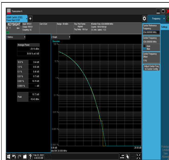
1-N5-PC3-15-20-L-4-DFT-64QAM-Outer_Full -100@0-8.46-100%-0.00-8.46-PASS-≤13
