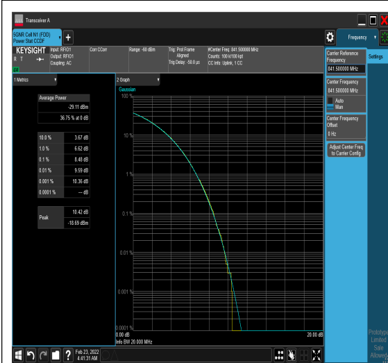
1-N5-PC3-15-15-H-1-DFT-PI2BPSK-Outter_F
