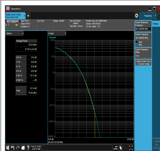
1-N5-PC3-15-15-H-9-CP-256QAM-Outer_Full-79@0-8.28-100%-0.00-8.28-PASS-≤13 1-N5-PC3-15-20-L-1-DFT-PI2BPSK-Outer_Full-100@0-8.41-100%-0.00-8.41-PASS-≤13
