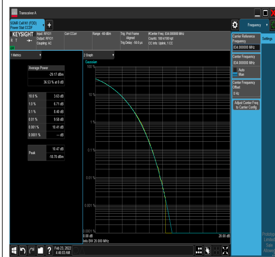
1-N5-PC3-15-20-L-8-CP-64QAM-Outer Full-
