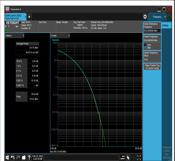
1-N5-PC3-15-15-H-9-CP-256QAM-Outer_Full-79@0-8.28-100%-0.00-8.28-PASS-≤13 1-N5-PC3-15-20-L-1-DFT-PI2BPSK-Outer_Full-100@0-8.41-100%-0.00-8.41-PASS-≤13
