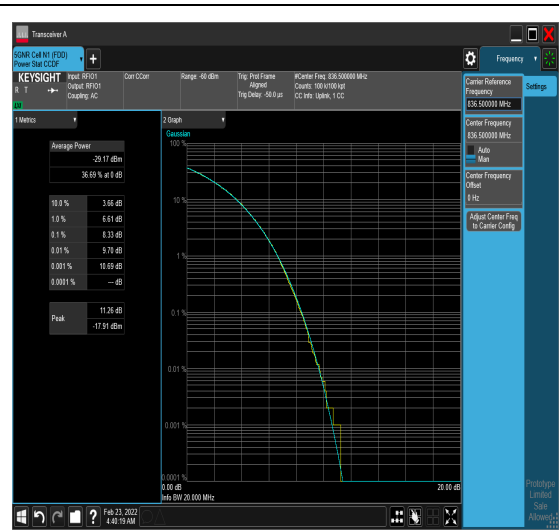
1-N5-PC3-15-15-M-7-CP-16QAM-Outter_Full-79 79@0-8.33-100%-0.00-8.33-PASS-≤13
