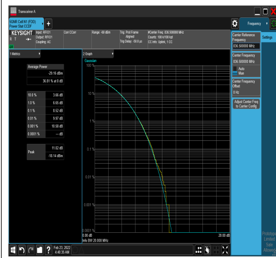
1-N5-PC3-15-15-M-8-CP-64QAM-Outter_Full-79 79@0-8.52-100%-0.00-8.52-PASS-≤13
