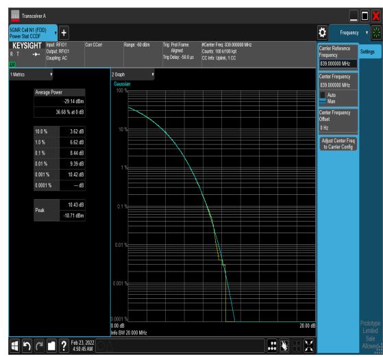
1-N5-PC3-15-20-H-5-DFT-256QAM-Outter_Full-100@0-8.44-100%-0.00-8.44-PASS-≤13
