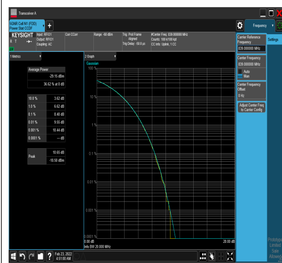
1-N5-PC3-15-20-H-6-CP-QPSK-Outter_Full-1
