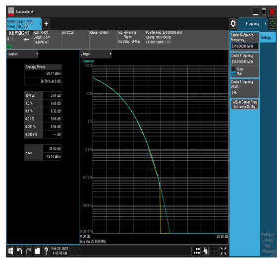
1-N5-PC3-15-20-L-7-CP-16QAM-Outer_Full- 106@0-8.32-100%-0.00-8.32-PASS-≤13
