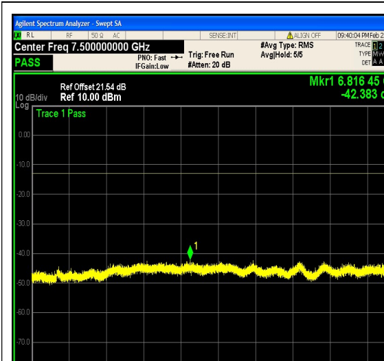
1-N5-PC3-15-10-L-10-DFT-64QAM-Edge_1R B_Left-1@0-3000-12000-Ant1--42.38--13-PA SS
