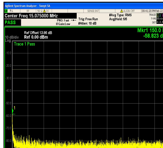
1-N5-PC3-15-10-L-12-DFT-64QAM-Outer_Fu ll-50@0.0.15-30-Ant1--58.82--23-PASS
