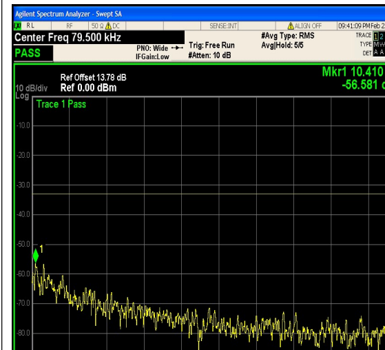
1-N5-PC3-15-10-L-12-DFT-64QAM-Outer_Fu ll-50@0-0.009-0.15-Ant1--56.58--33-PASS
