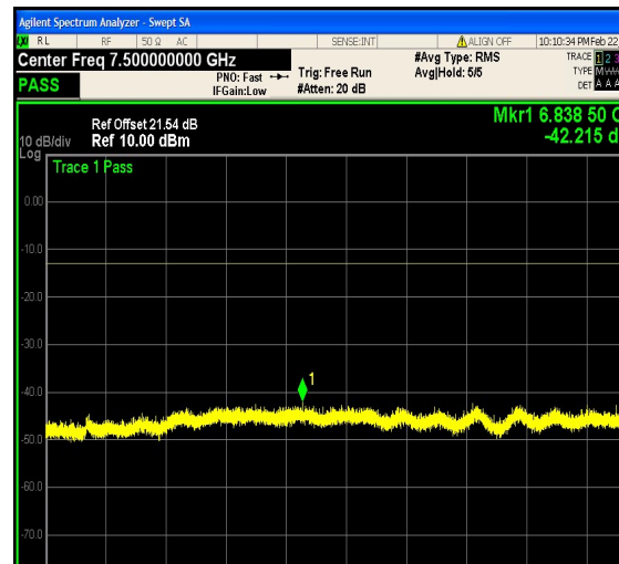
1-N5-PC3-15-10-M-8-DFT-16QAM-Edge_1R B_Right-1@51-3000-12000-Ant1--42.21--13- PASS
