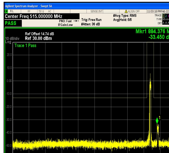
1-N5-PC3-15-10-H-15-DFT-256QAM-Outer_ Full-50@0-30-1000-Ant1--33.45--13-PASS
