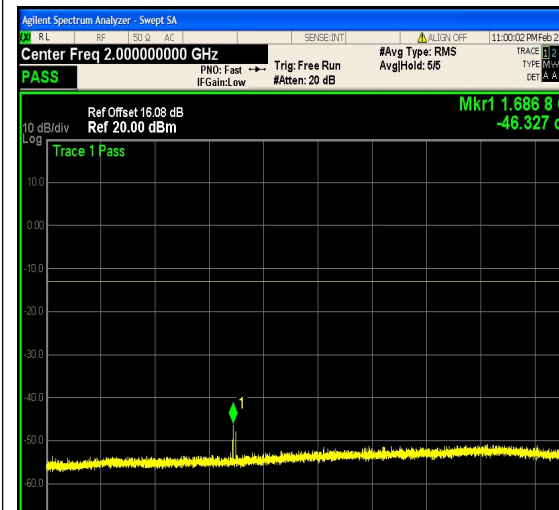
1-N5-PC3-15-10-H-11-DFT-64QAM-Edge_1R B_Right-1@51-1000-3000-Ant1--46.33--13-P ASS
