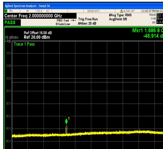
1-N5-PC3-15-10-H-14-DFT-256QAM-Edge_1 RB_Right-1@51-1000-3000-Ant1--46.91--13- PASS
