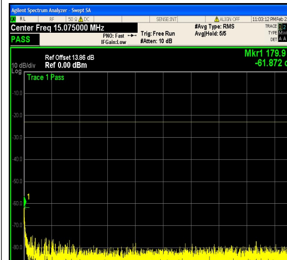
1-N5-PC3-15-10-H-15-DFT-256QAM-Outer_ Full-50@0-0.15-30-Ant1--61.87--23-PASS
